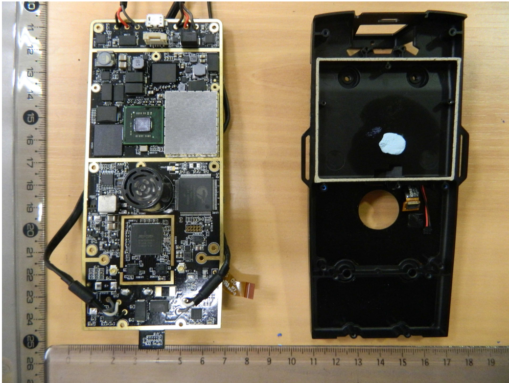
Mother Board (Top)
