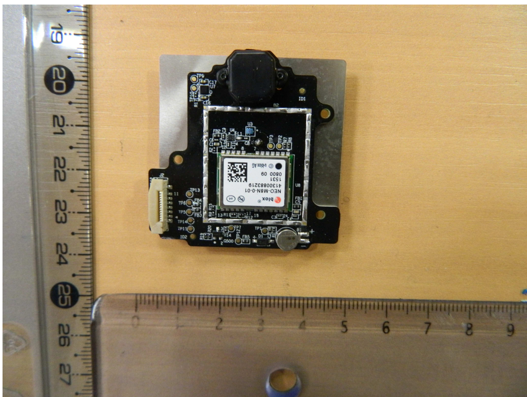
GNSS board(Top)
