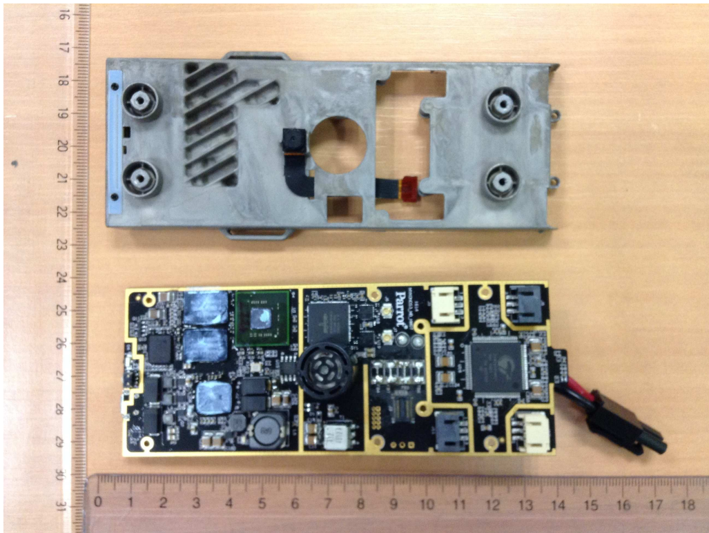
Mother Board without shield (Top)
