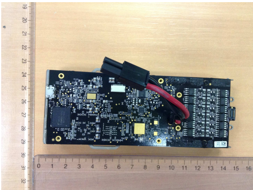
Mother Board (Bottom)
