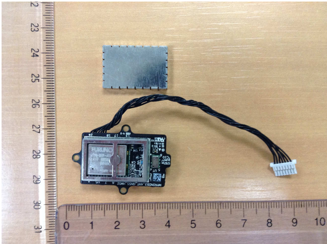
Antenna GNSS without shield (Top)
