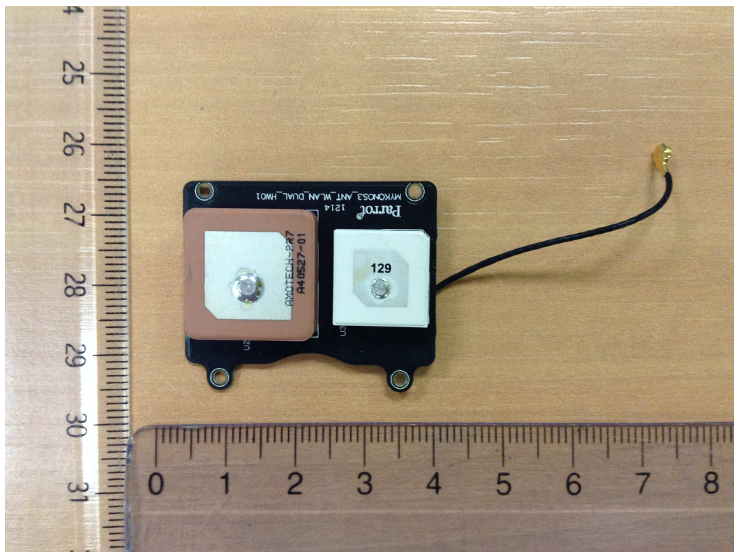
Antenna WLAN (Bottom)
