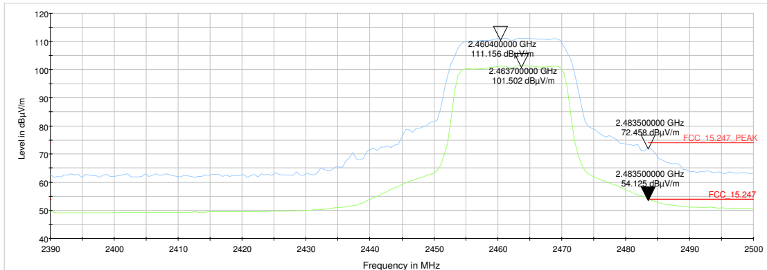
Delta-marker Radiated pre measurement
