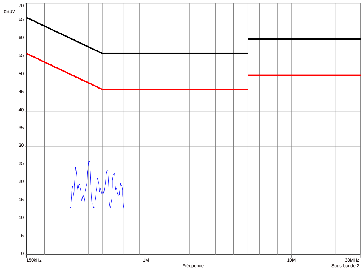
Average measurement on the Line from 300 kHz to 700 kHz
