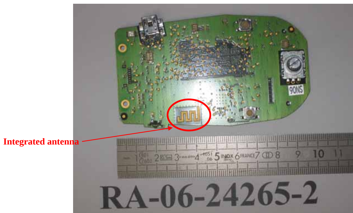
Printed circuit board: face 2
