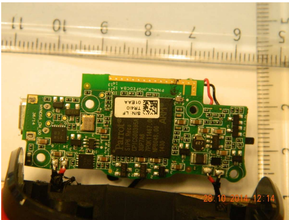
BOTTOM VIEW
