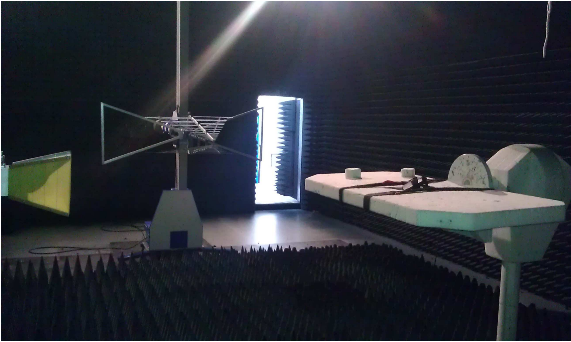
Photo 3: Test setup for radiated measurements (Enclosure, fully-anechoic chamber, 1-18 (15) GHz intentional radiator §15)
