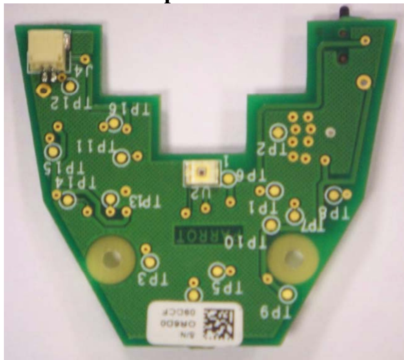
OROS Receptacle board Bottom
