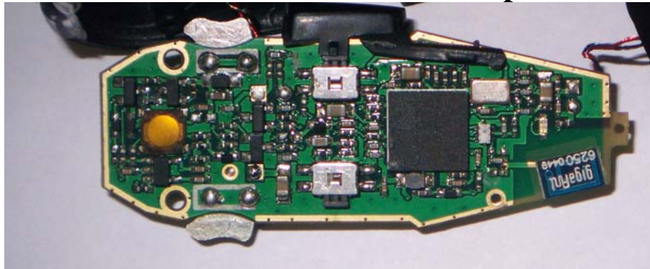
OROS Headset board Bottom
