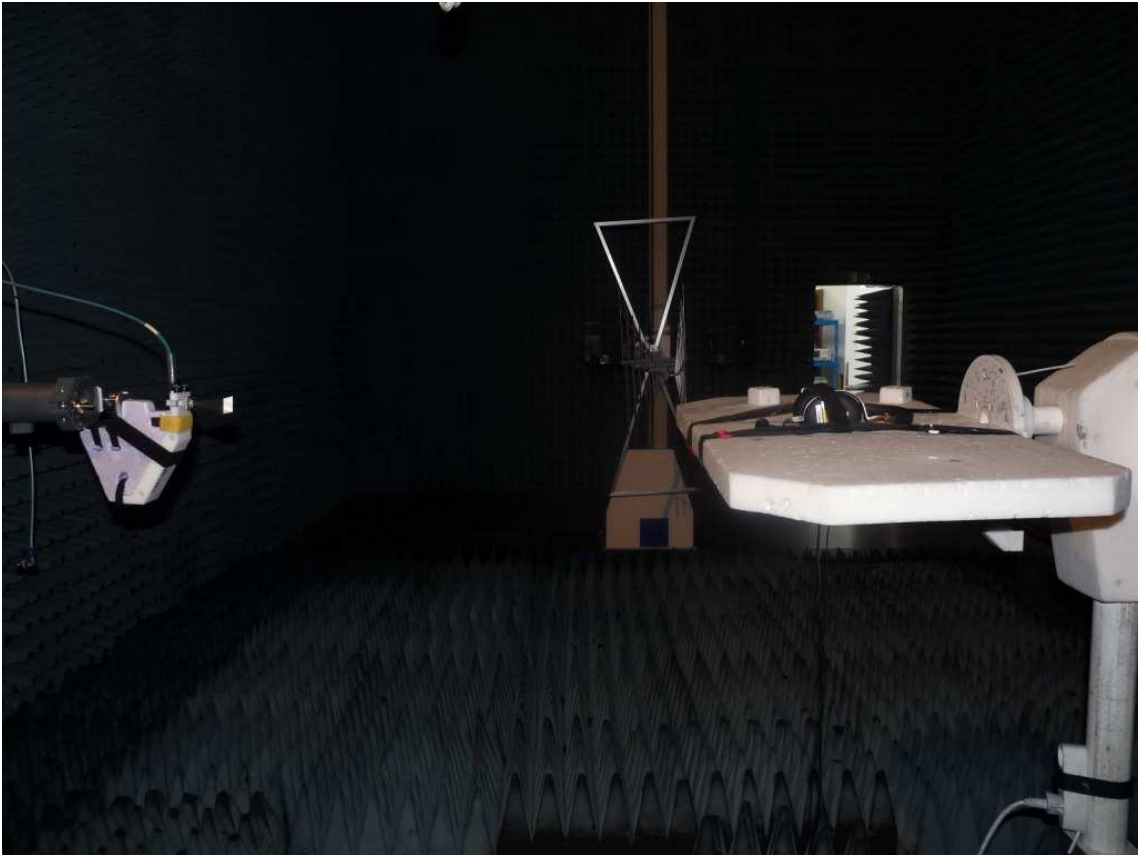
Photo 4: Test setup for radiated measurements (18 GHz up to 25 GHz)
