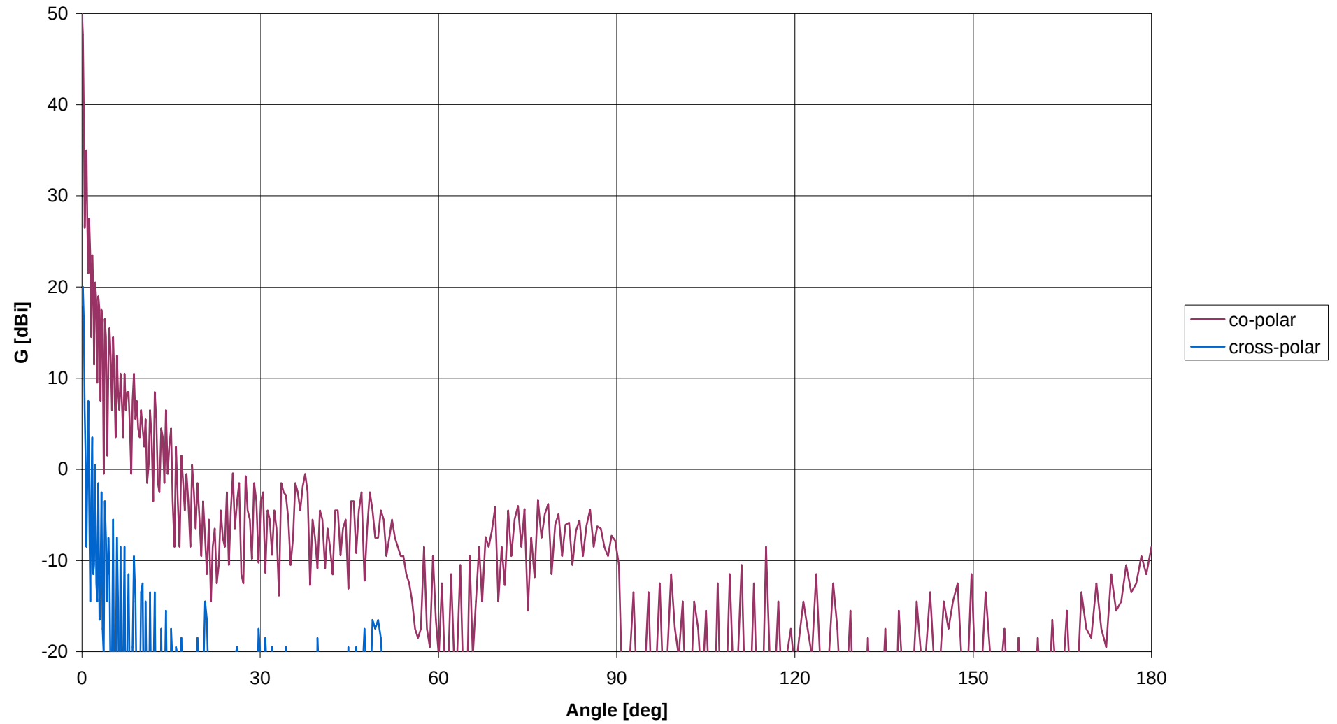
Radiation Pattern Performance. 73.5 GHz, 0.6m
