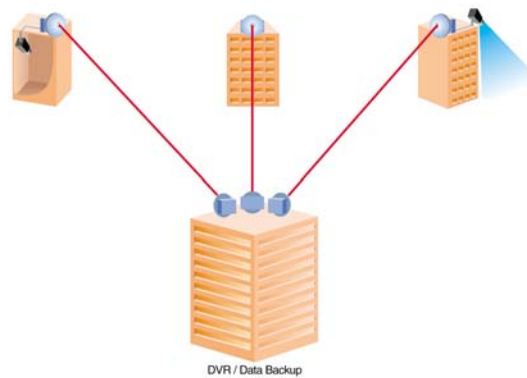
Figure 1-6 Security & Internet
