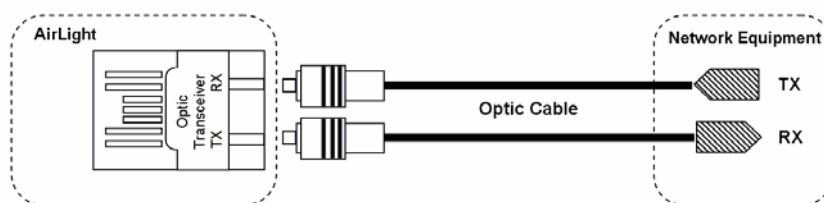
Figure 3-1 Network Connection
