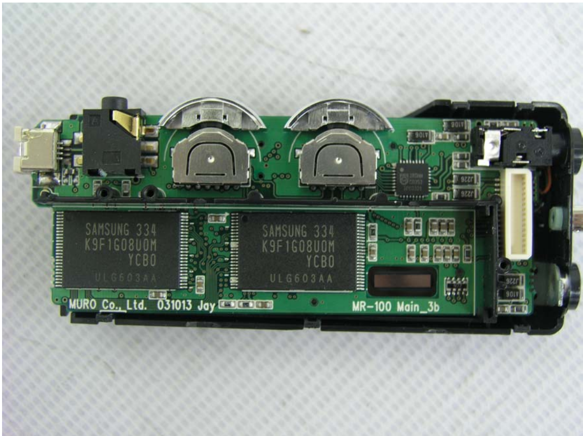
Main board
