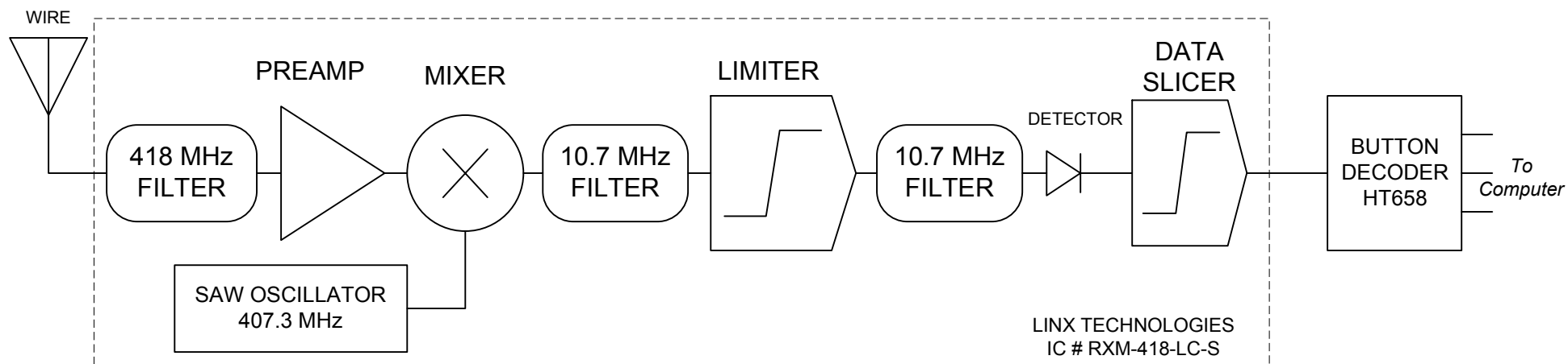
RECEIVER BLOCK DIAGRAM
