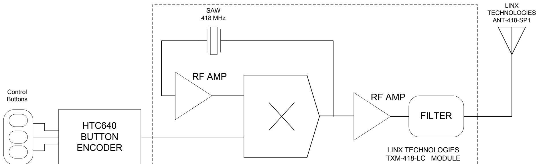
TRANSMITTER BLOCK DIAGRAM
