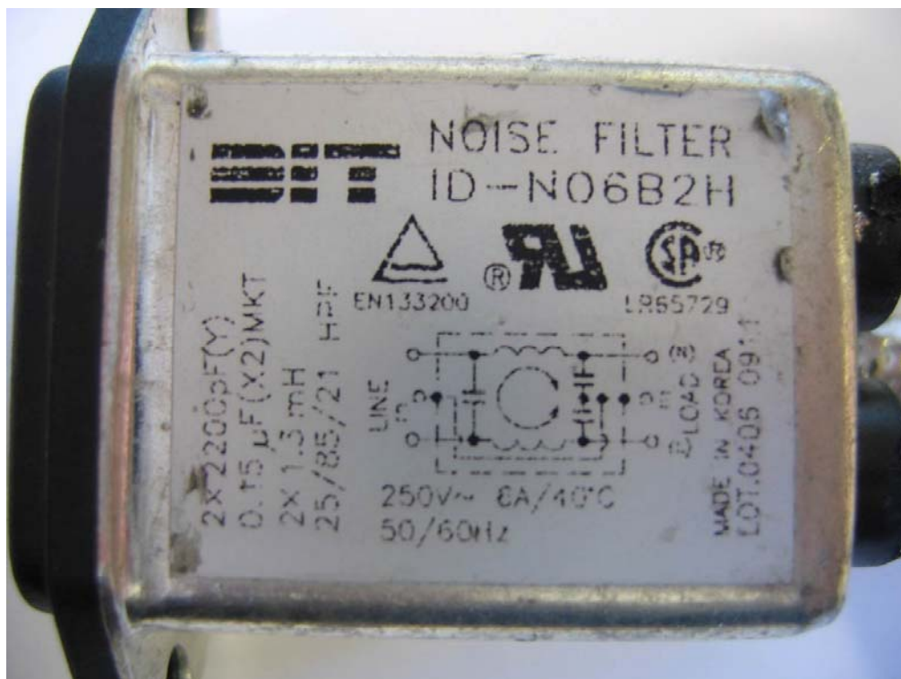
(Noise filter model : ID-N06B2H, manufacturer : DIT)
