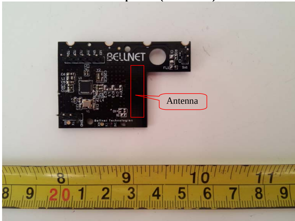
EUT –Top View (BN-BP210)
