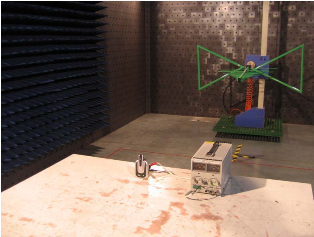
Radiated Emission (Charging mode)
