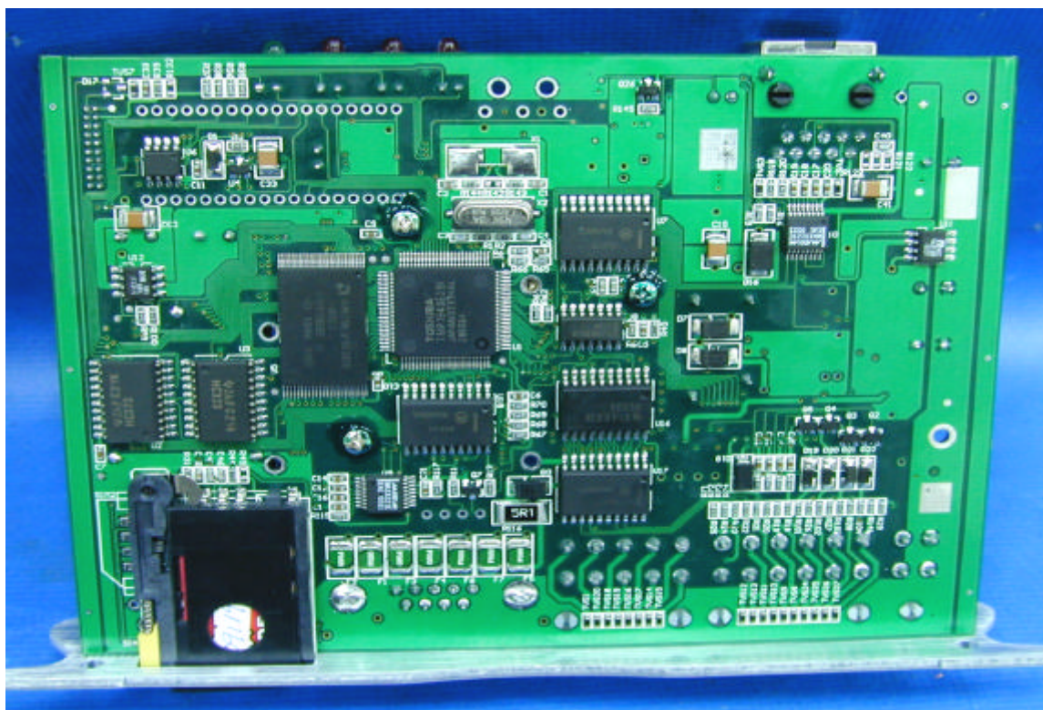
PHOTO. 6. EUT SOLDERING SIDE VIEW
