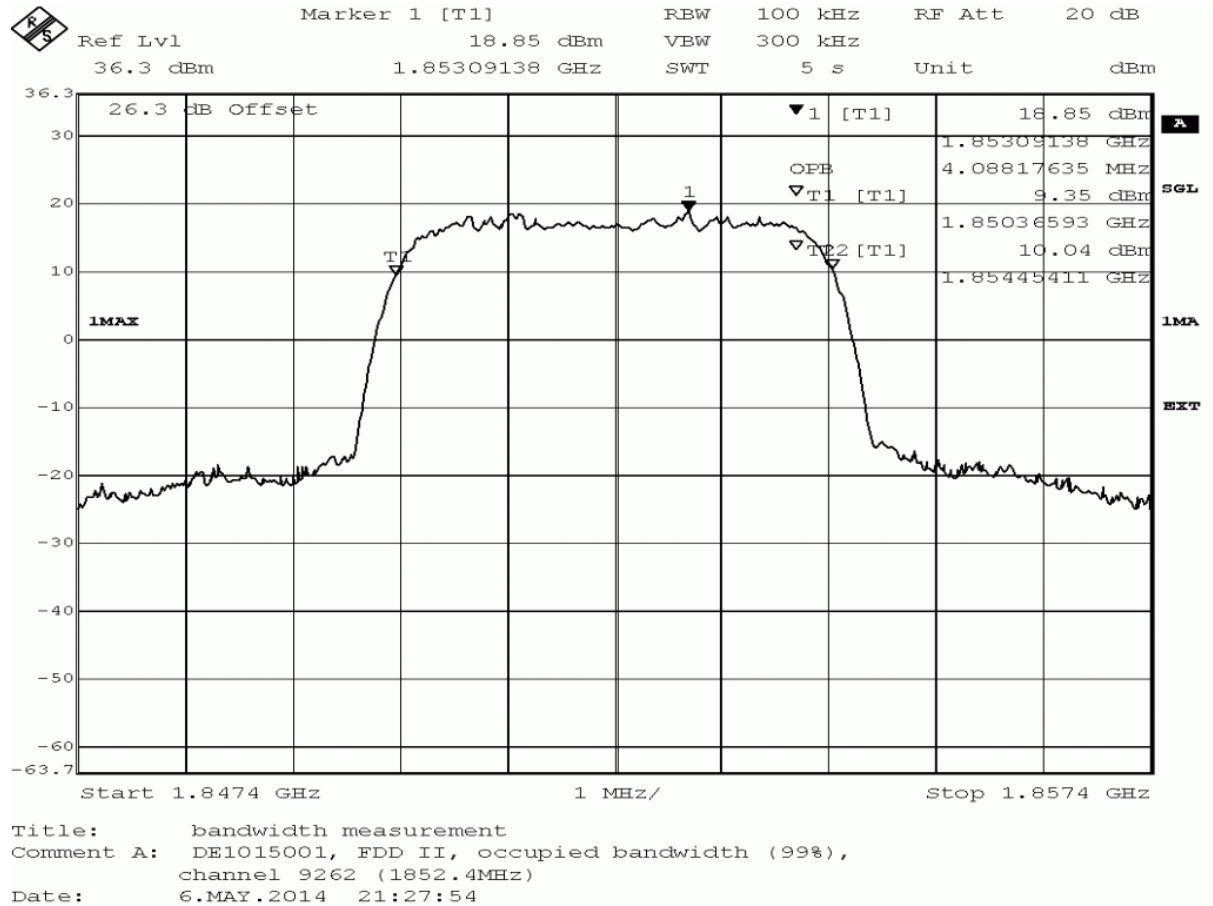
HSDPA 99% Bandwidth Low Channel
