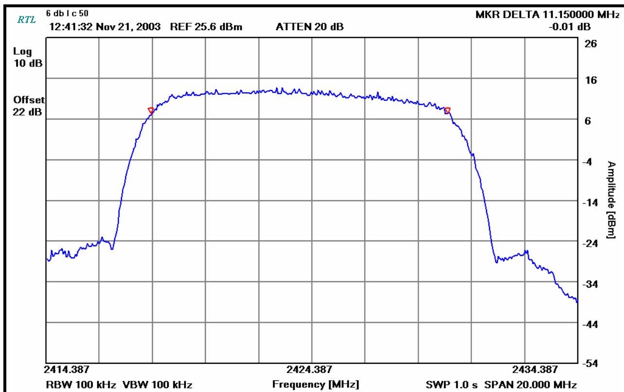
PLOT 7-3: MODULATED BANDWIDTH MIDDLE CHANNEL AT 50 MBPS
