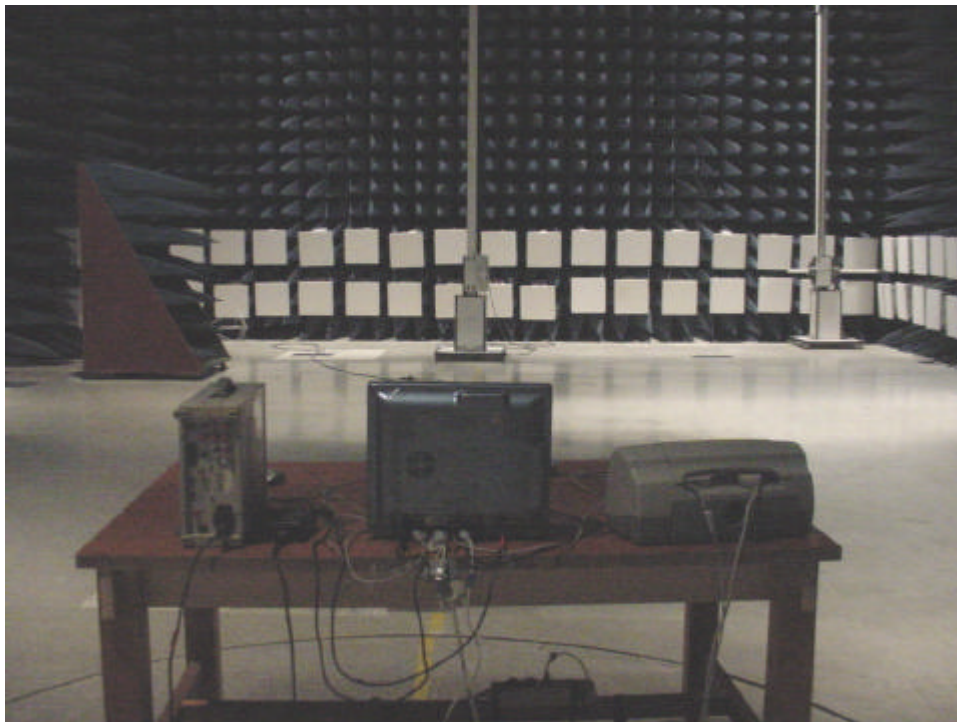
<REAR PHOTO OF RADIATED DISTURBANCE >
