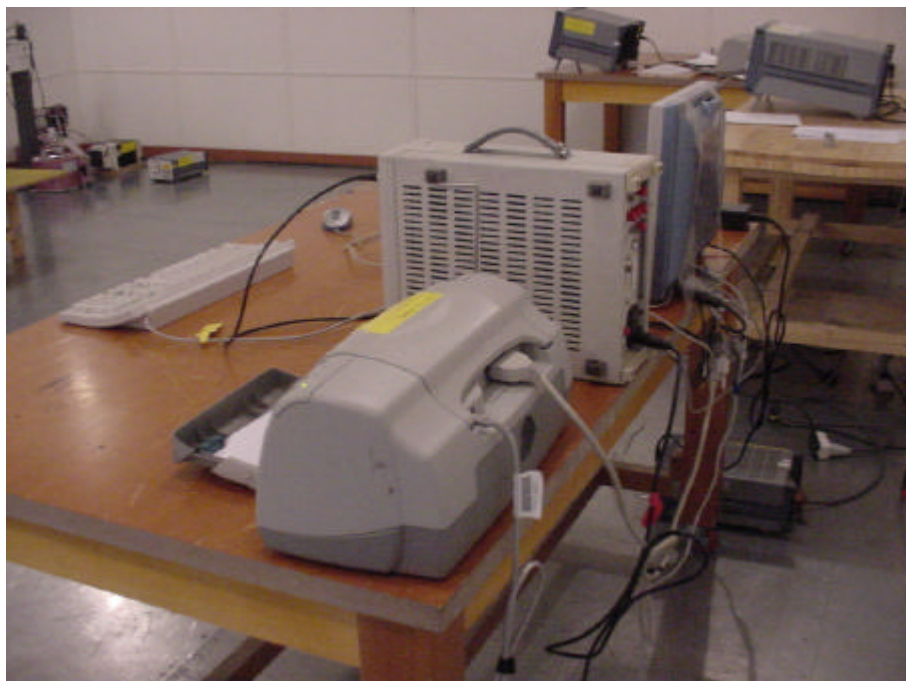
<SIDE PHOTO OF CONTINUOUS DISTURBANCE VOLTAGE >
