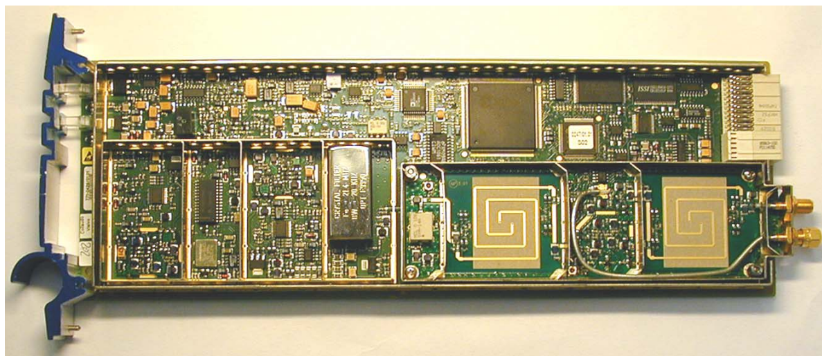
Figure 1 - Module RX – internal view of receiver
