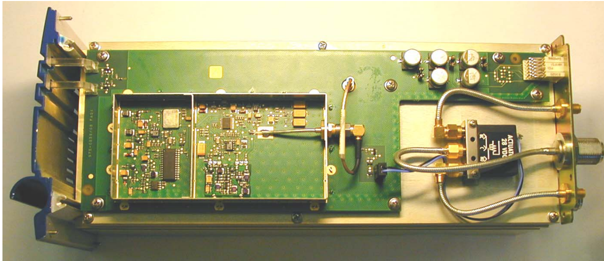
Figure 2 - Module TX- - internal view of transmitter
