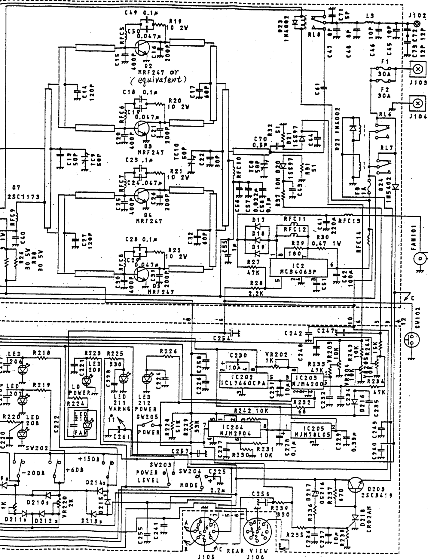
HL-350VDX CIRCUIT DIAGRAM
