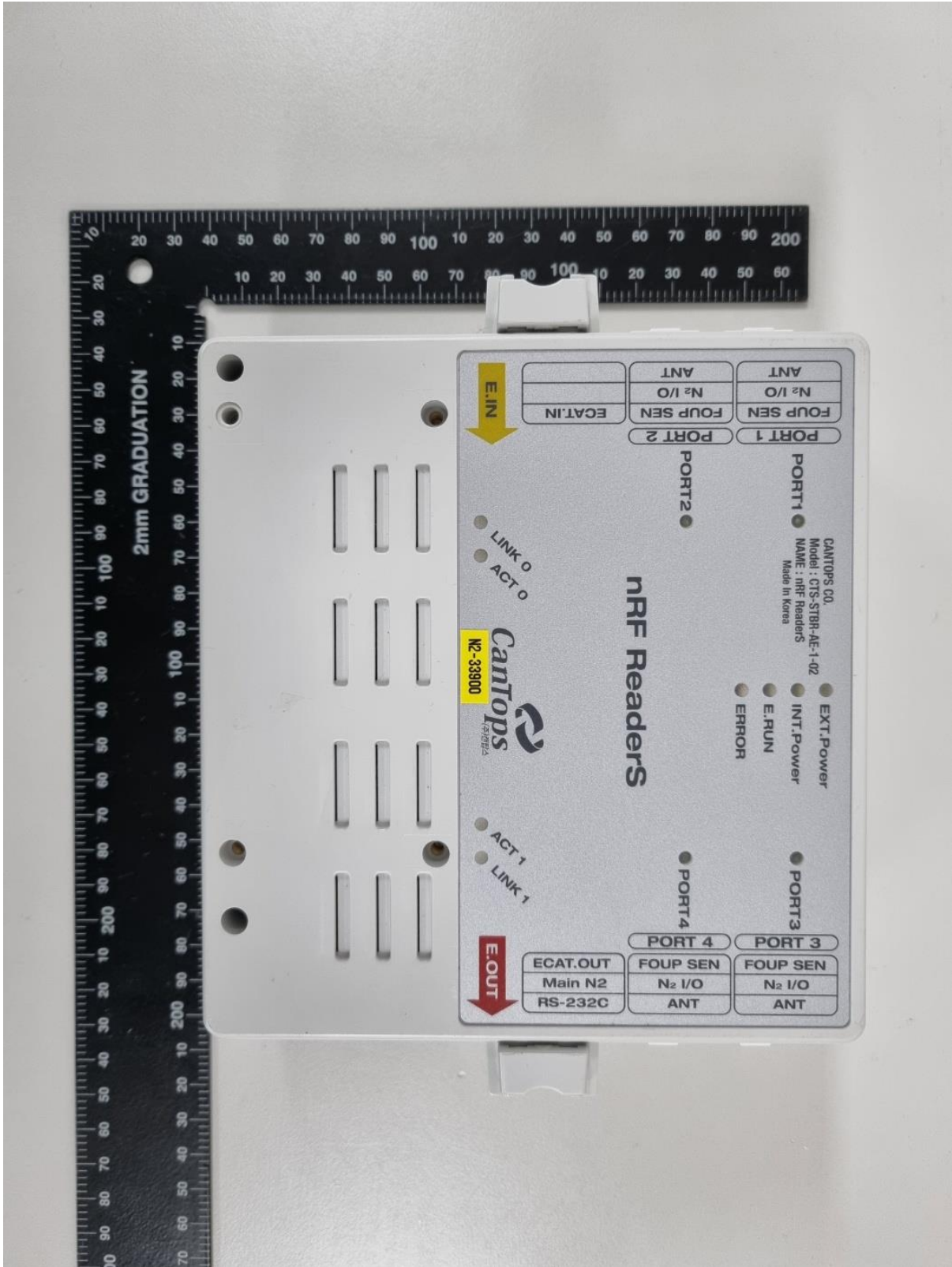
Front
