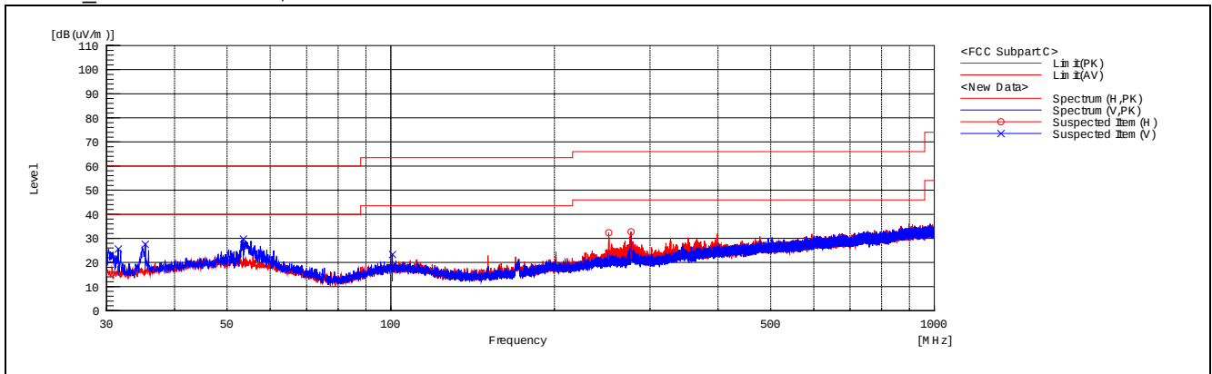
Port 2_External antenna, 2 405 MHz
