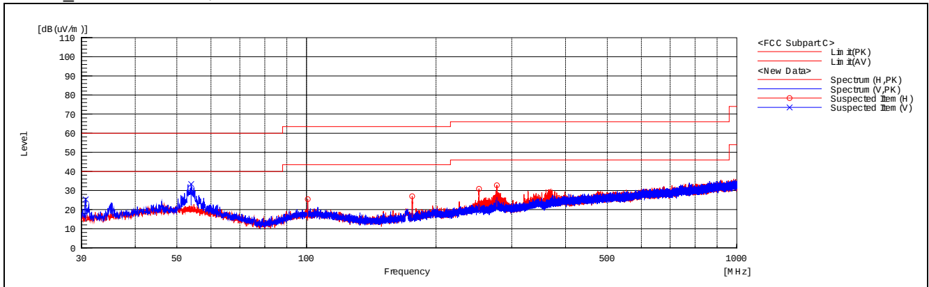
Port 2_Internal antenna, 2 405 MHz
