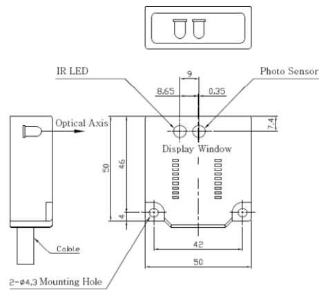
< F Type : Front View >
