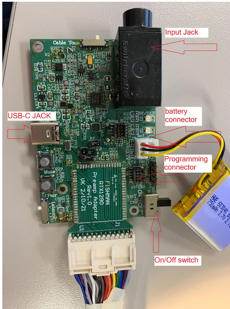
Figure 3: motherboard support board
