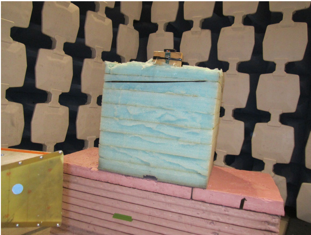
Radiated Spurious Emission, 6 – 18GHz
