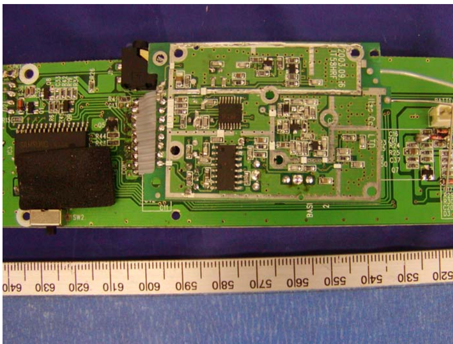
Handset – Transceiver Solder View
