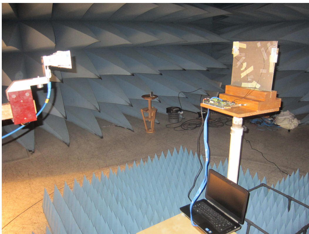
Fig. 5. Test set-up for radiated measurements above 18GHz to 25GHz
