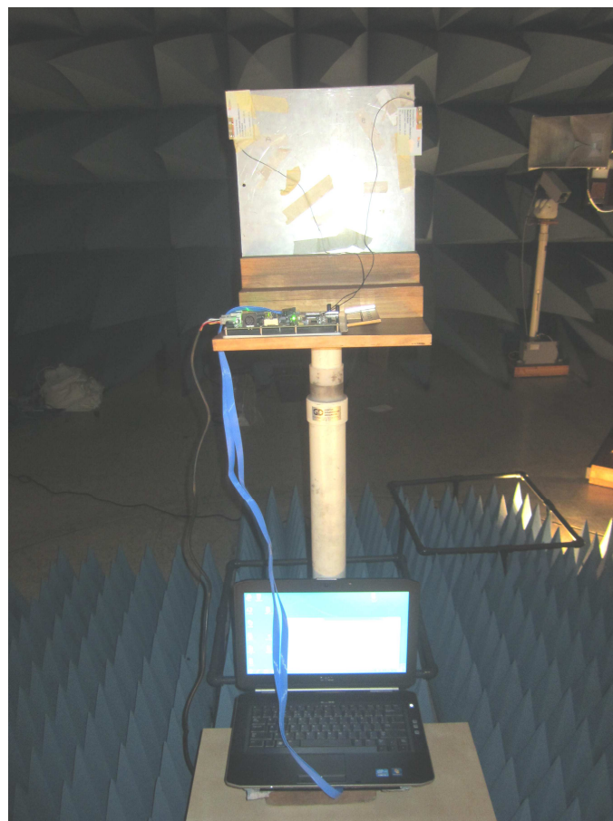
Fig. 3. Antenna frontal view
