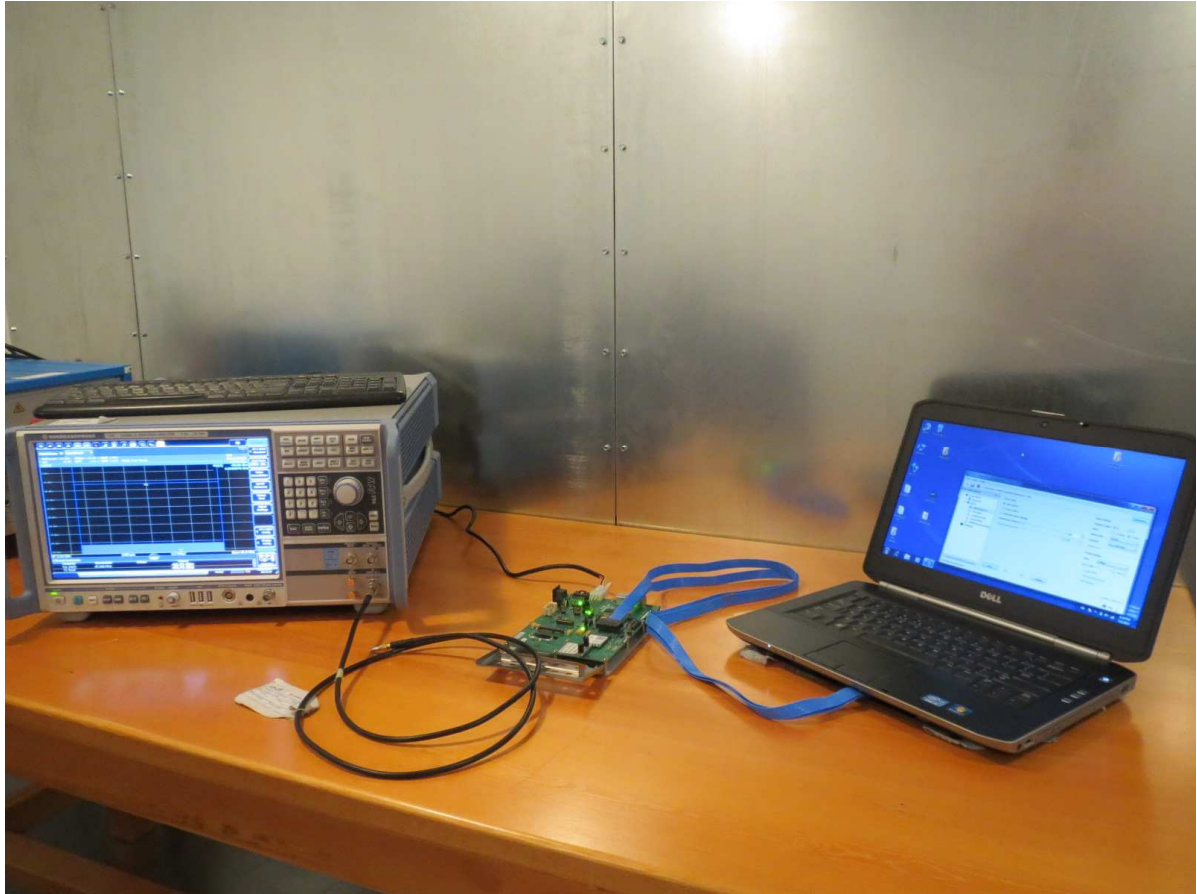
Fig. 6. Test set-up for conducted measurements
