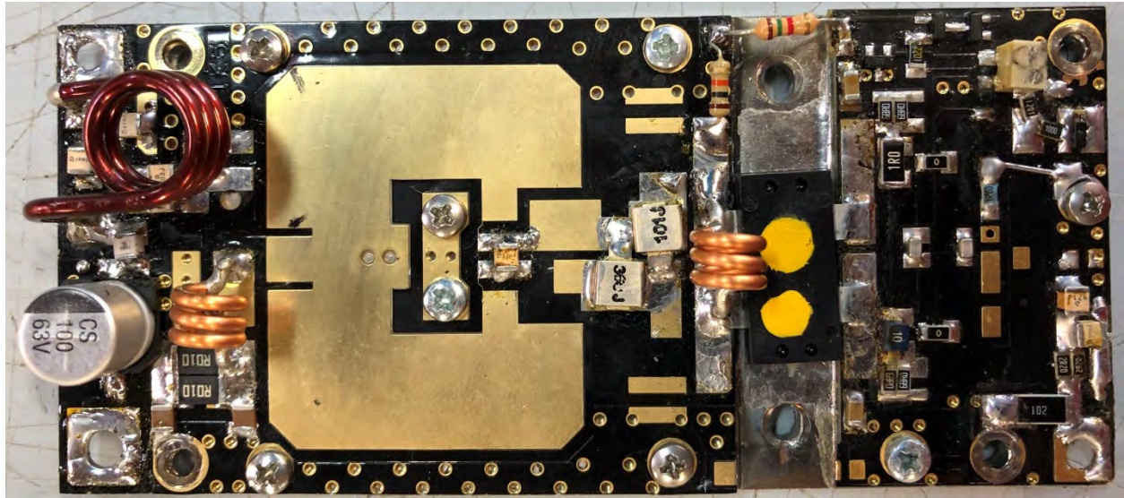
RF PALLET BOARD – FRONT VIEW
