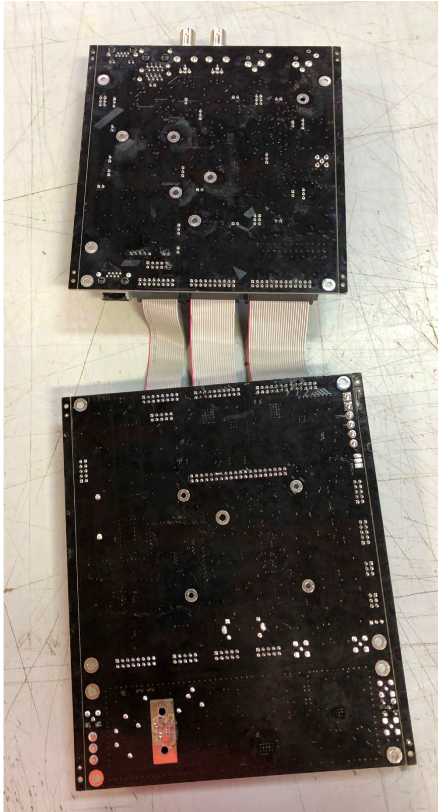
MOTHER BOARD – REAR VIEW
