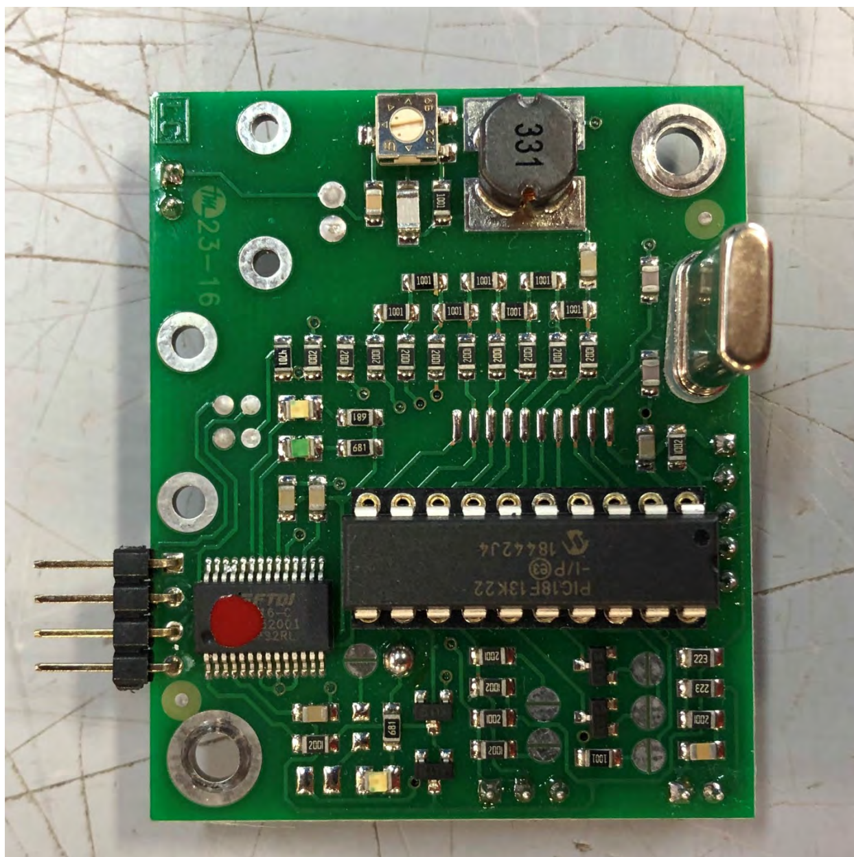
RDS BOARD – FRONT VIEW
