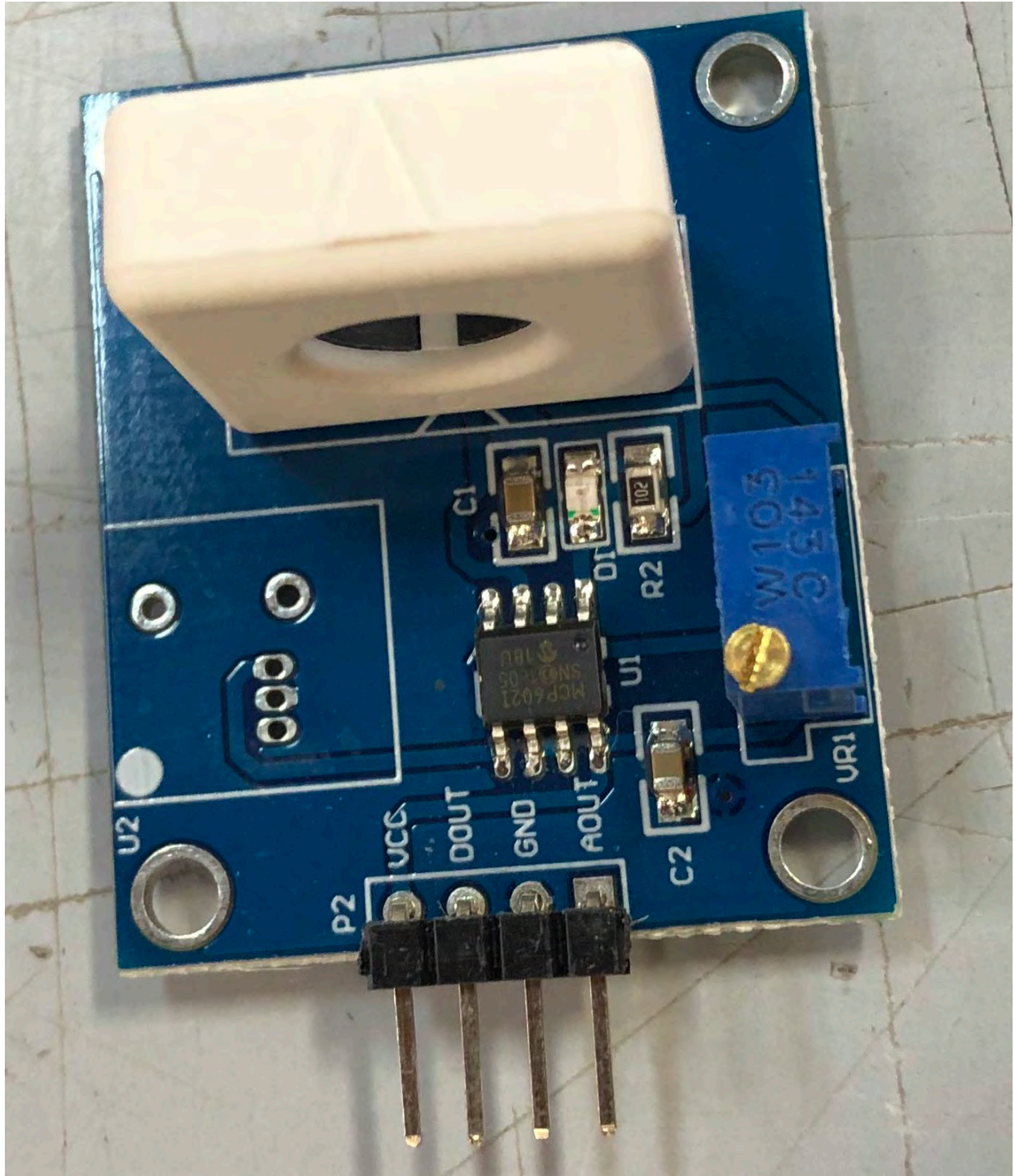
CURRENT READING BOARD – FRONT VIEW
