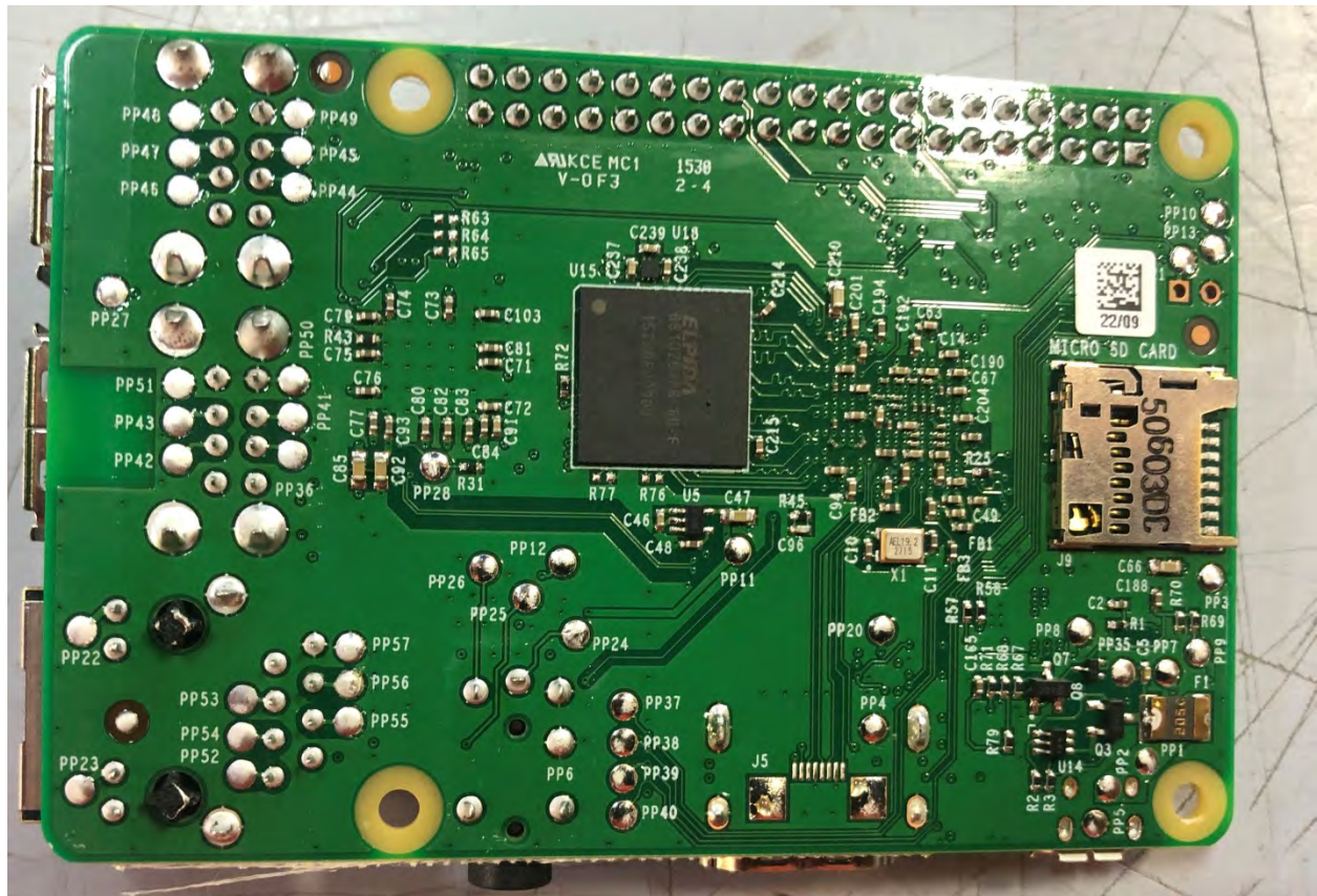
RASBERRY PI BOARD – REAR VIEW
