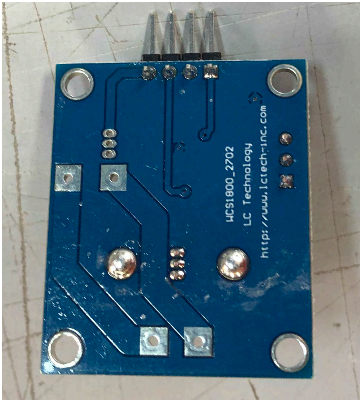
CURRENT READING BOARD – REAR VIEW
