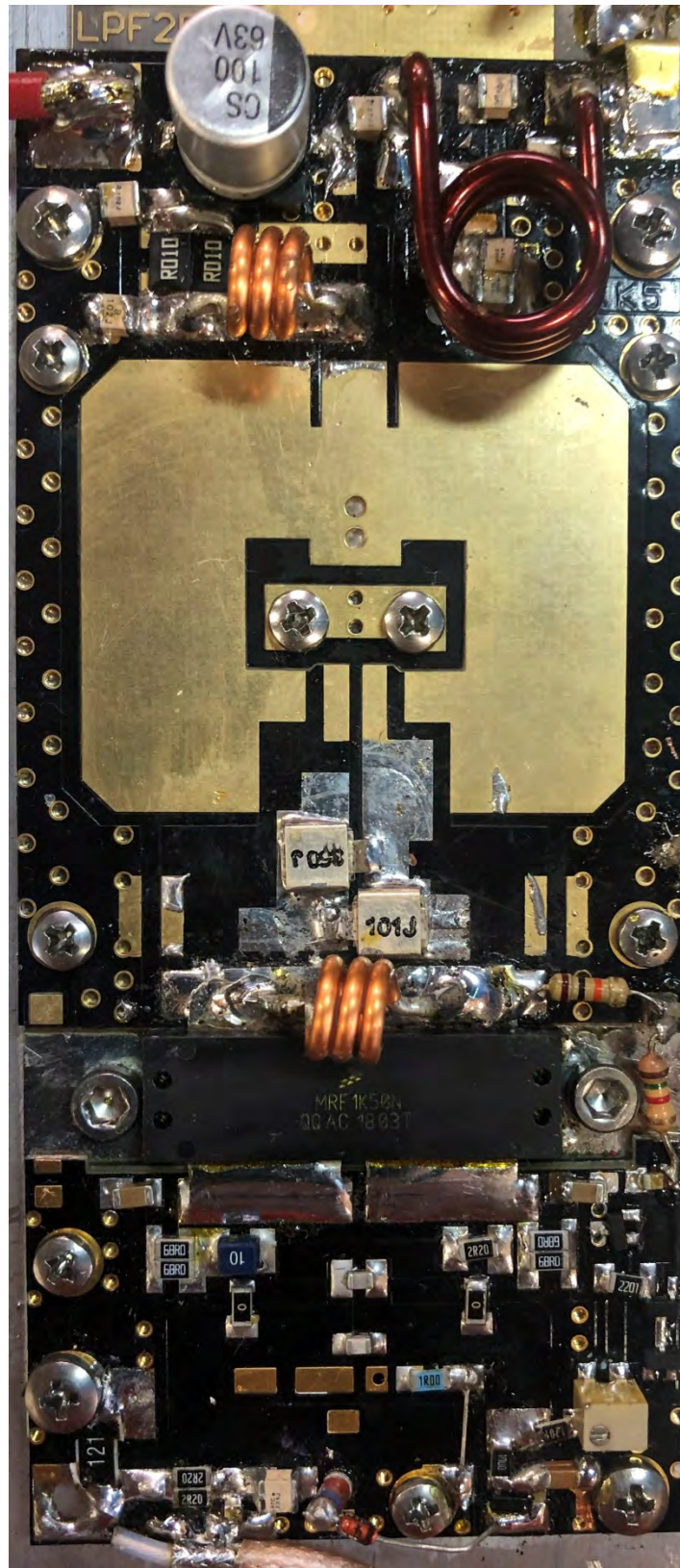
RF PALLET BOARD – FRONT VIEW
