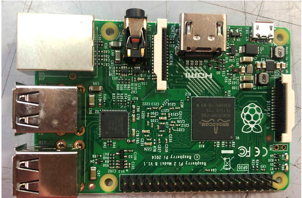
RASBERRY PI BOARD – FRONT VIEW
