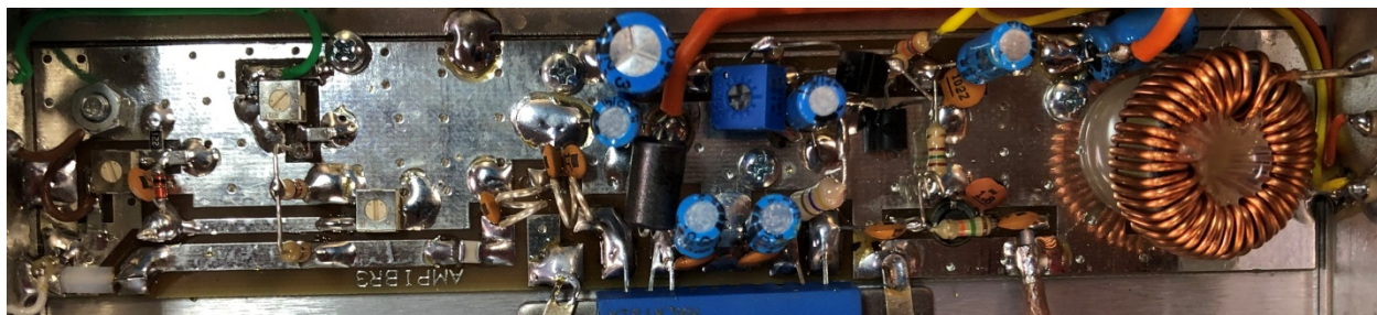
AMPLIFIER BOARD – FRONT VIEW
