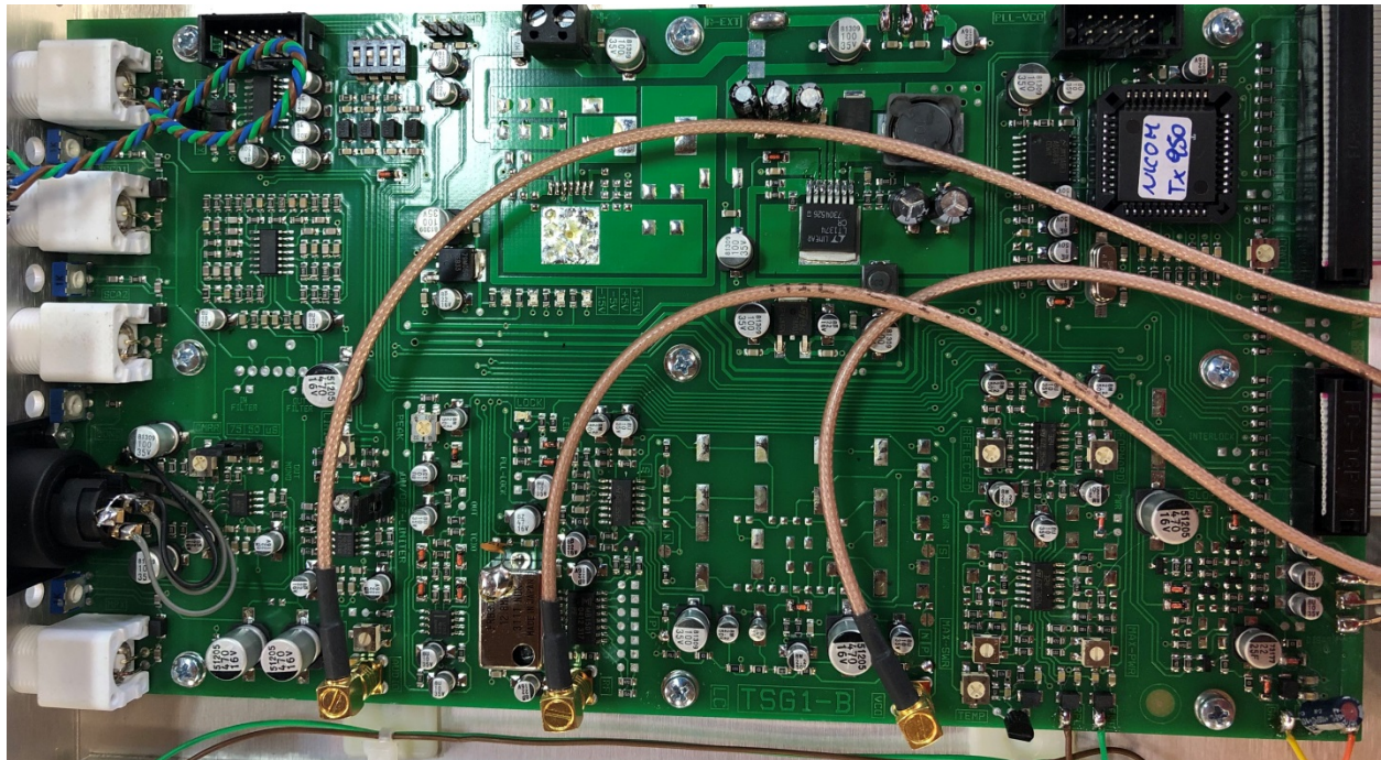
MOTHERBOARD – FRONT VIEW
