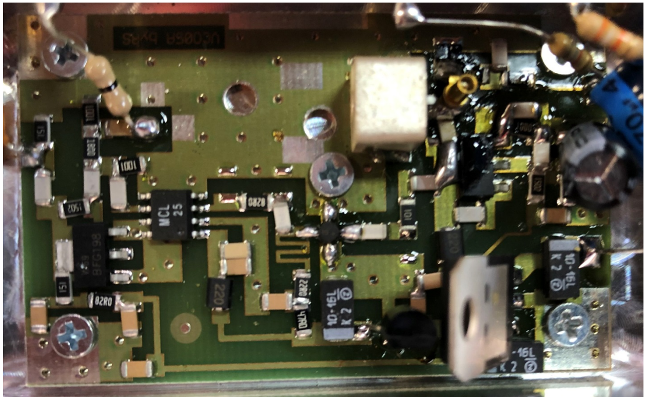
VCO BOARD – FRONT VIEW
