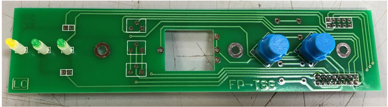
CONTROL BOARD – FRONT VIEW
