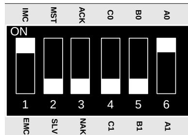
Figure 3-1: DVModule Manual DIP Switch Configuration (Example: Slave Mode)
