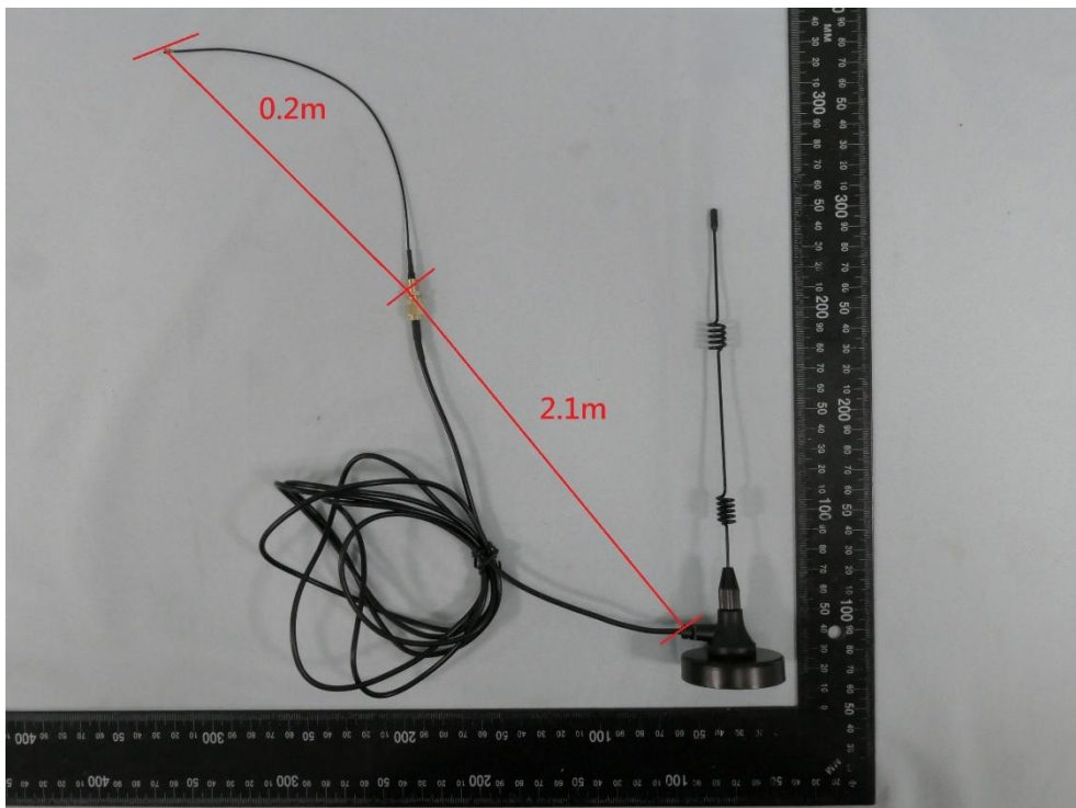
(18) EUT Photo (M/N: MP.54.2400.228)
