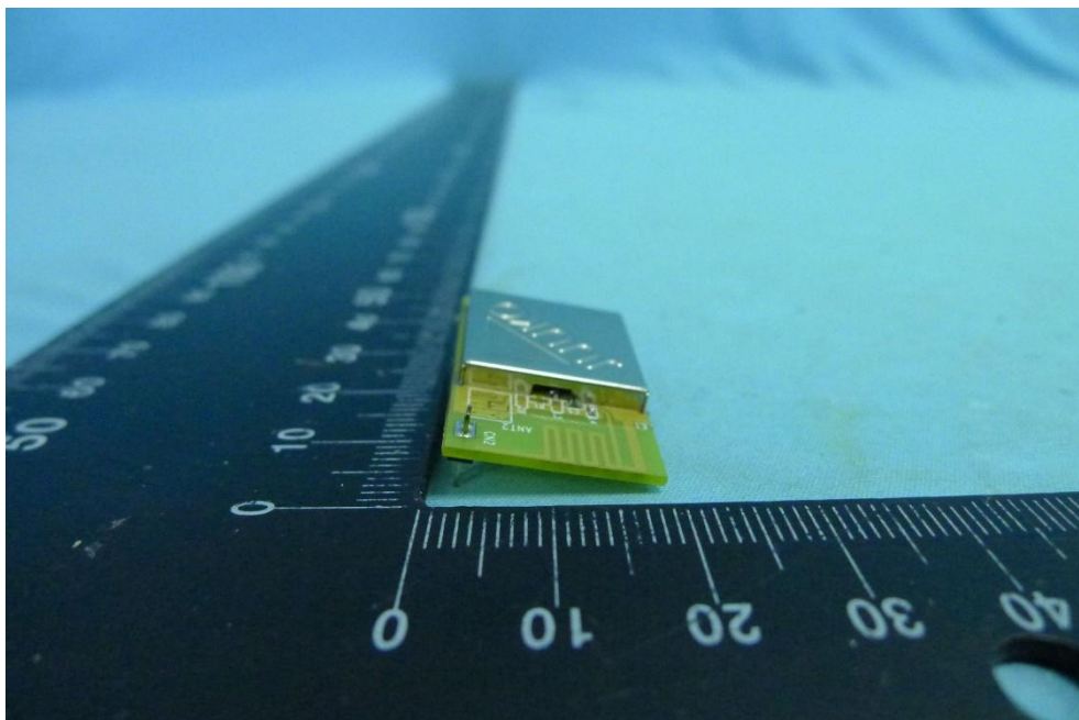
(6) EUT Photo ( for Internal Antenna)
