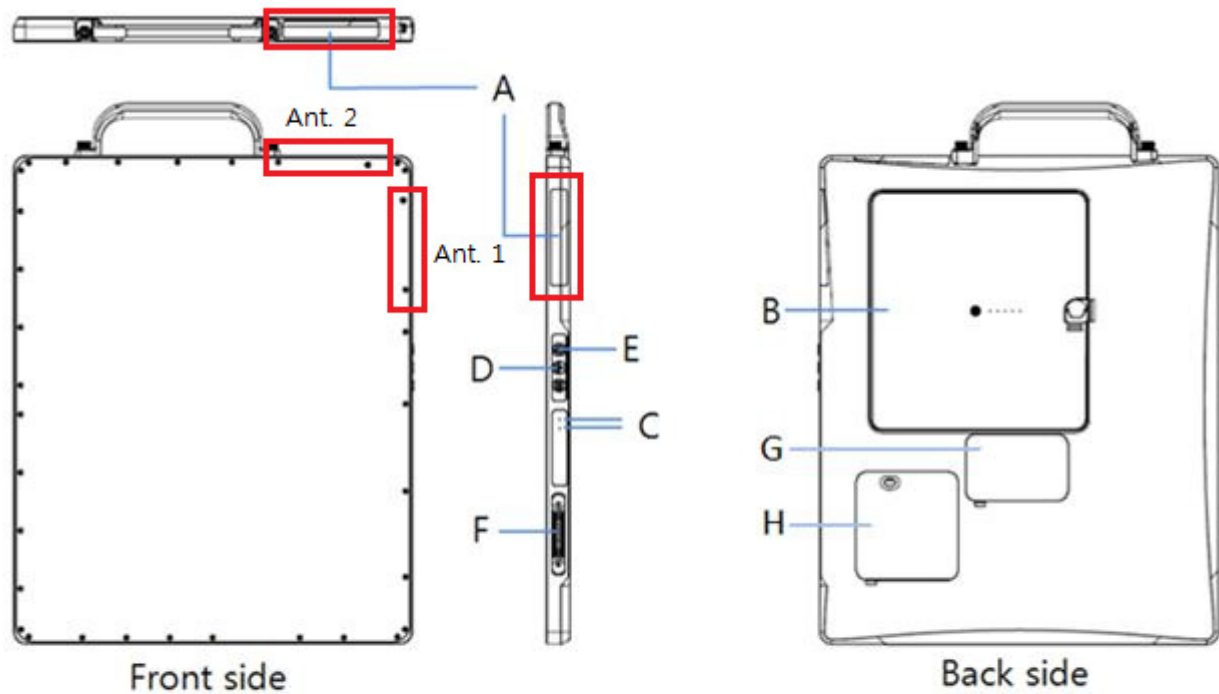
Figure 4.1. Detector Components
