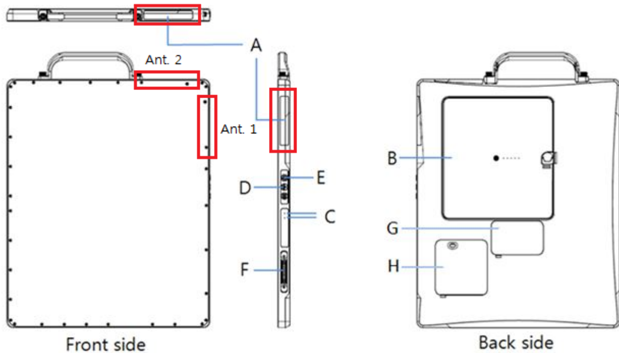
Figure 4.1. Detector Components
