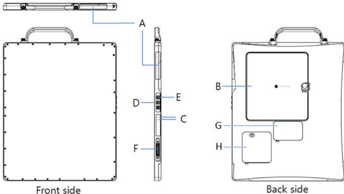
Figure 4.1. Detector Components
