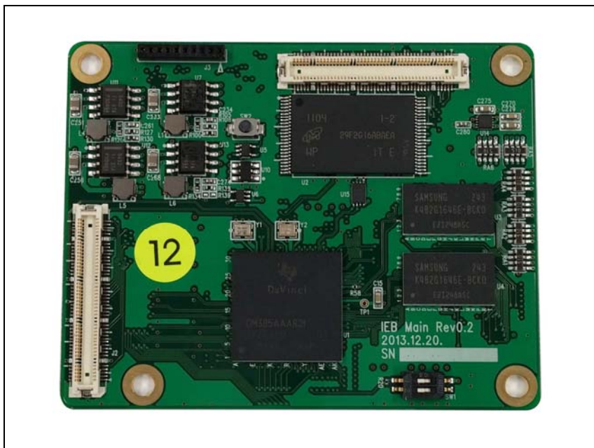
Embedded board(Top)
