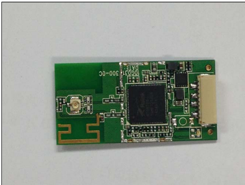
RF Module(Shields removed_Top)
