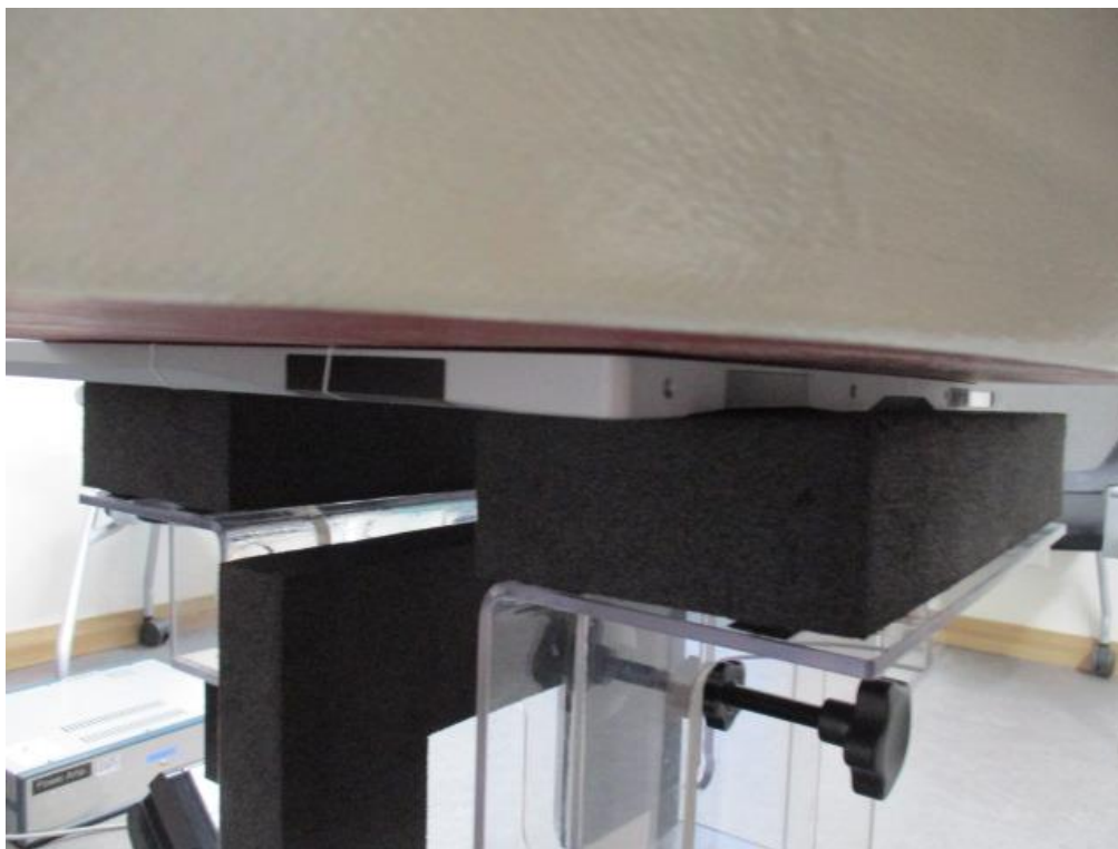
Front Side from Flat Phantom (Separation Distance: 0 cm)_Ant.1+2 (MIMO)
