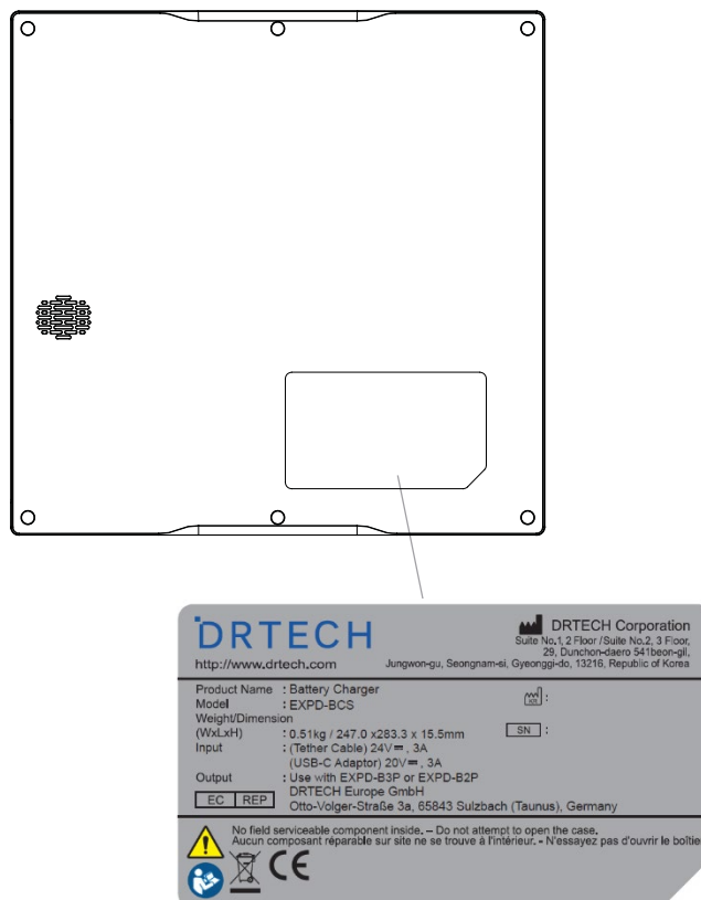
Figure 5. Product Label and Marking position of the Battery Charger(EXPD-BCS)
