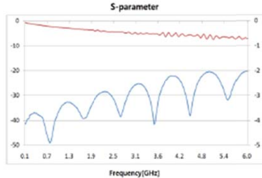
CMP25(G)-G113-CMP25(G)-100mm
