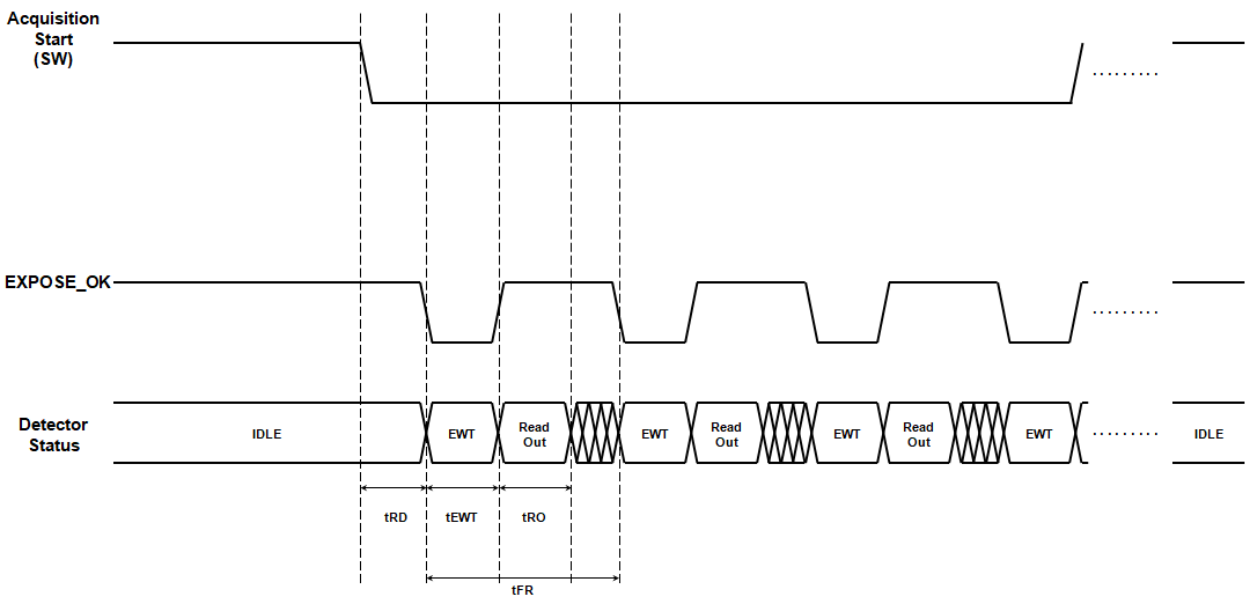
Figure 22. Timing Diagram for the Multi-frame Internal type
