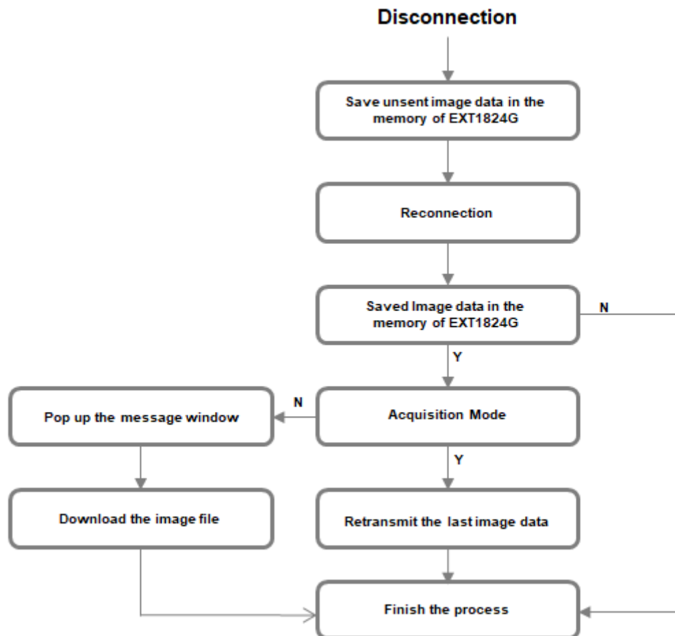
Figure 5.2. Flow Chart
