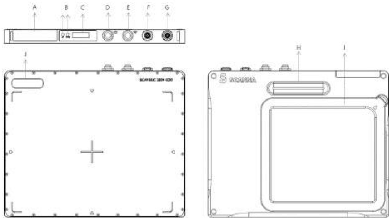
Figure 4.1. Detector Components
