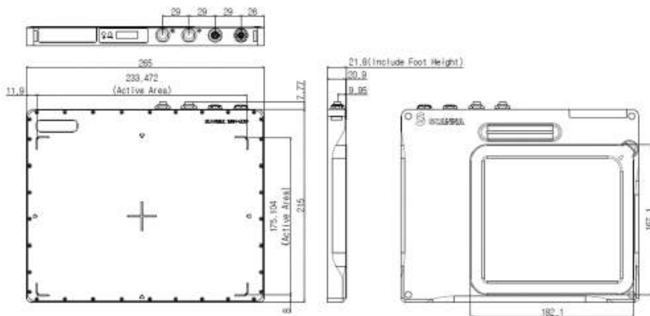
Figure 10.1 Detector Dimension
