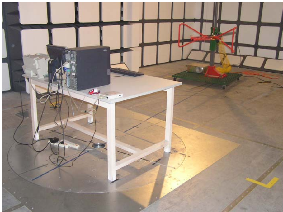
Charging mode: Radiated Emission-Rear View
