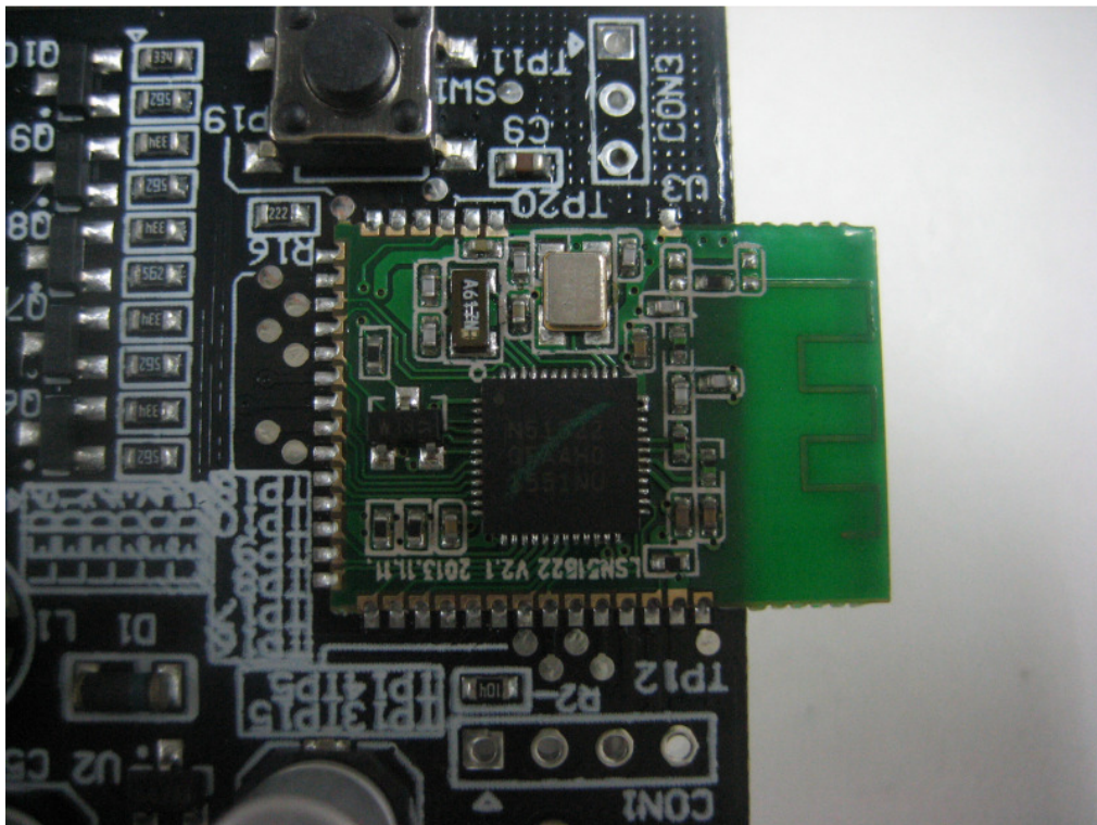
Internal View (Model: WRT2-RX)
