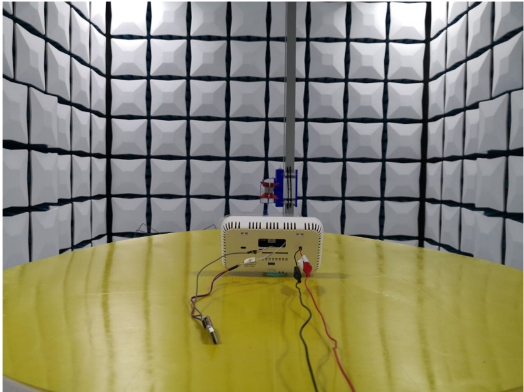
Set-up for Radiated Emission (worst case)
