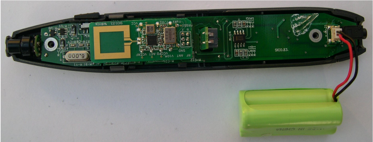
<Photograph 1: Cover removed>
