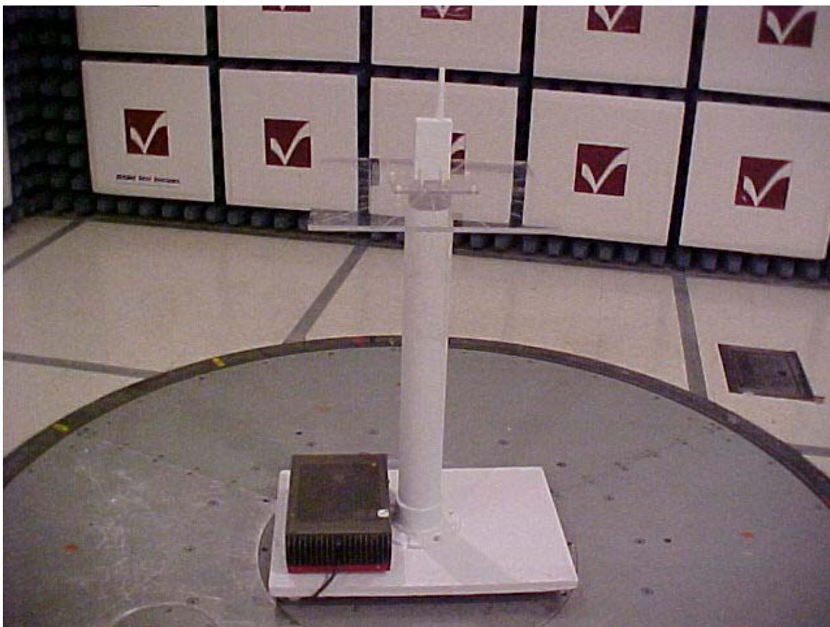
Setup of the EUT with the external DC power supply, in the semi-anechoic chamber, during the radiated emission testing.
