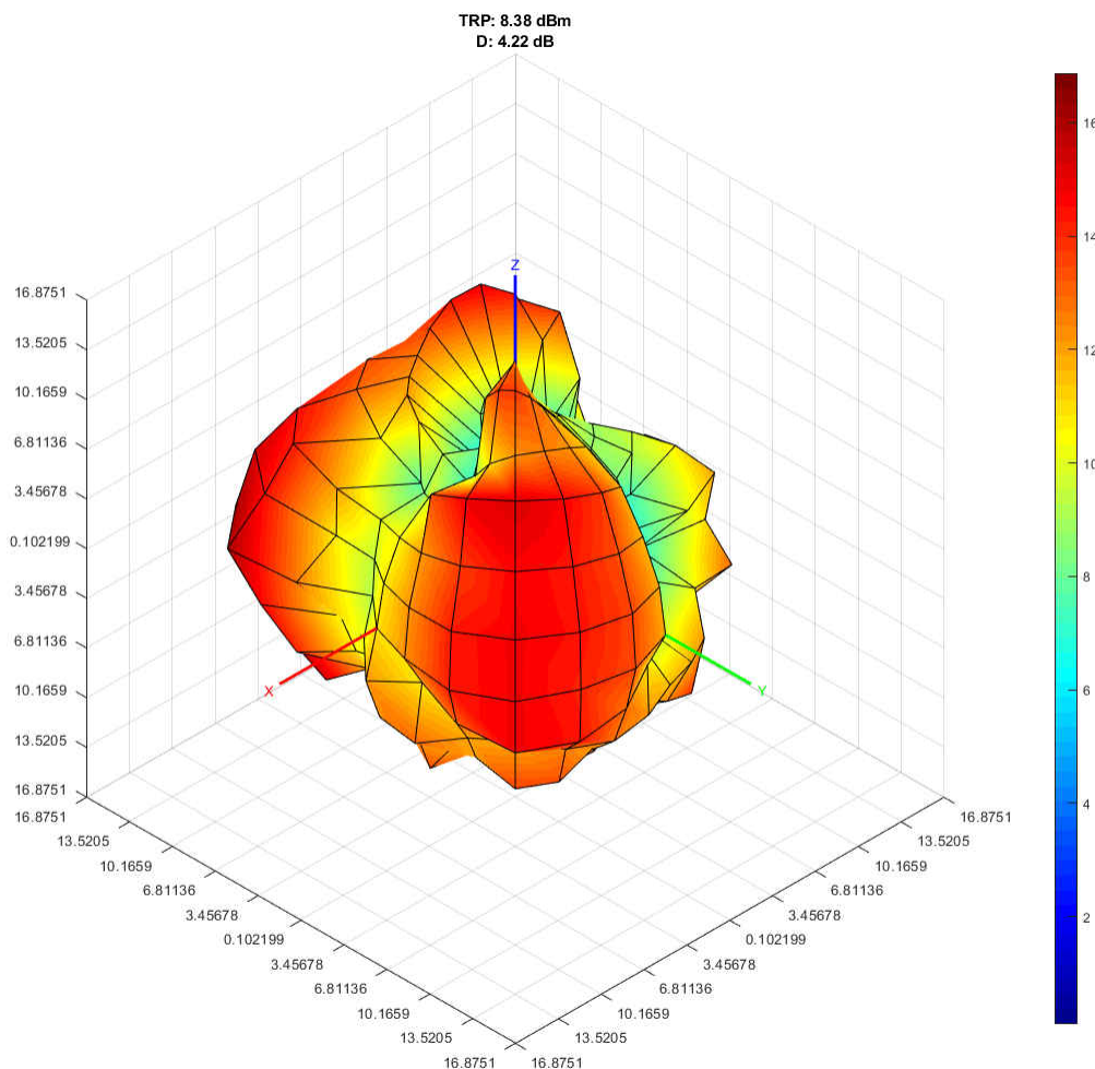
Figure 5-31. Radiation Pattern of the Antenna Matched for Dual-Band 868/915 and 2440-MHz Radiating with 10-dBm 2440-MHz Setting
