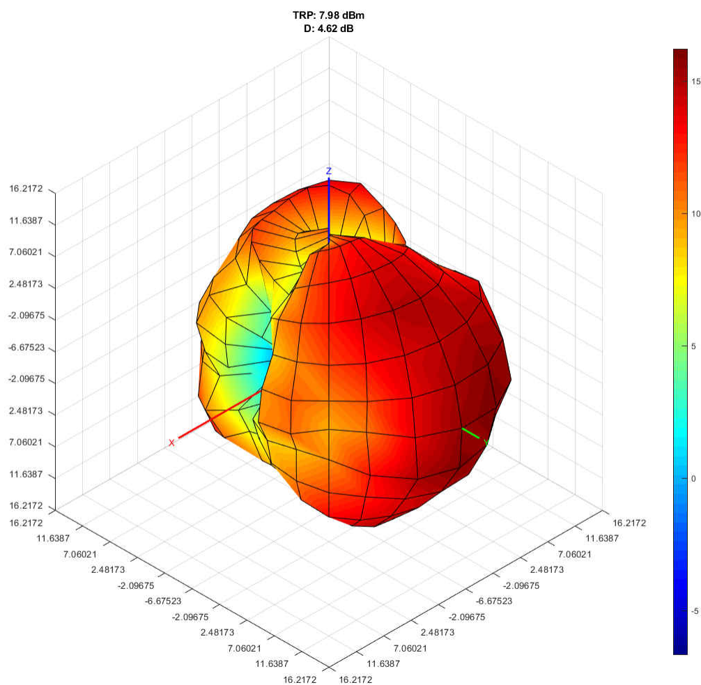
Figure 5-18. Radiation Pattern of the Antenna Matched for Dual-Band 490 and 2440-MHz Radiating with 10-dBm 2440-MHz Setting
