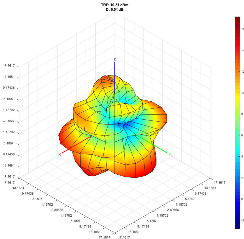
Figure 4-20. Radiation Pattern of the Antenna Matched for 892-MHz Radiating with 13 dBm 868-MHz Setting
