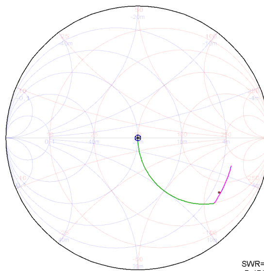
Figure 5-20. Theoretical Smith Chart for Dual Band 2440 MHz Match
