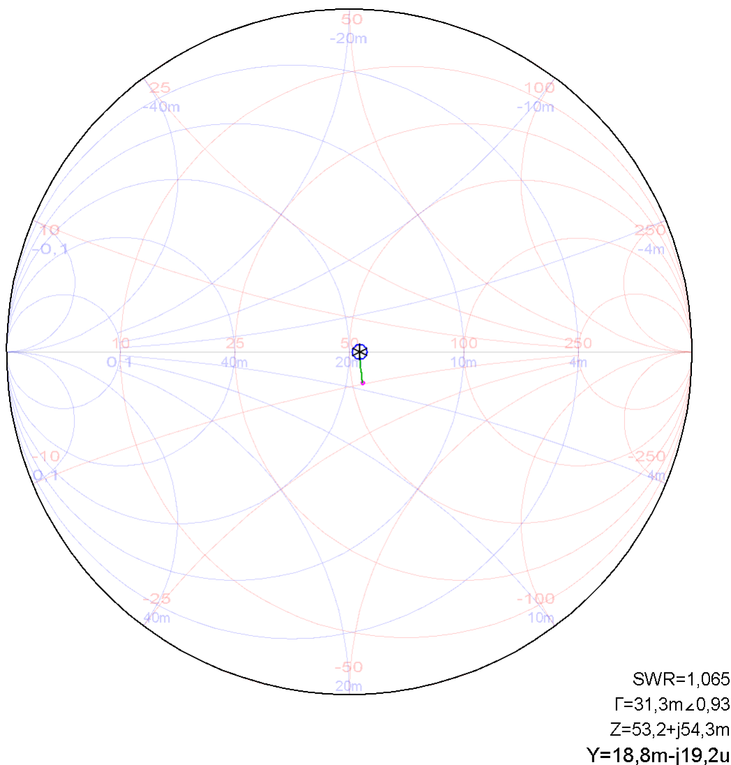
Figure 4-17. Theoretical Smith Chart for Single-Band 892-MHz Matching
