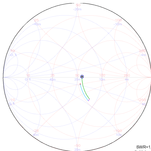
Figure 5-25. Theoretical Smith Chart for Dual-Band 892-MHz Match
