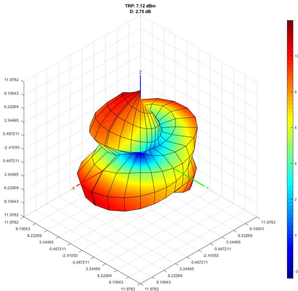
Figure 5-17. Radiation Pattern of the Antenna Matched for Dual-Band 490 and 2440 MHz Radiating with 13 dBm 490 MHz Setting
