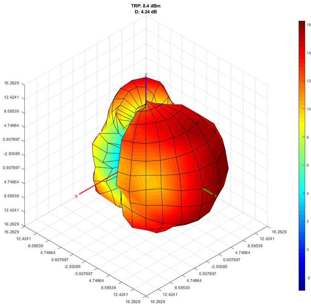
Figure 5-24. Radiation Pattern of the Antenna Matched for Dual-Band 510 and 2440-MHz Radiating with 10-dBm 2440-MHz Setting
