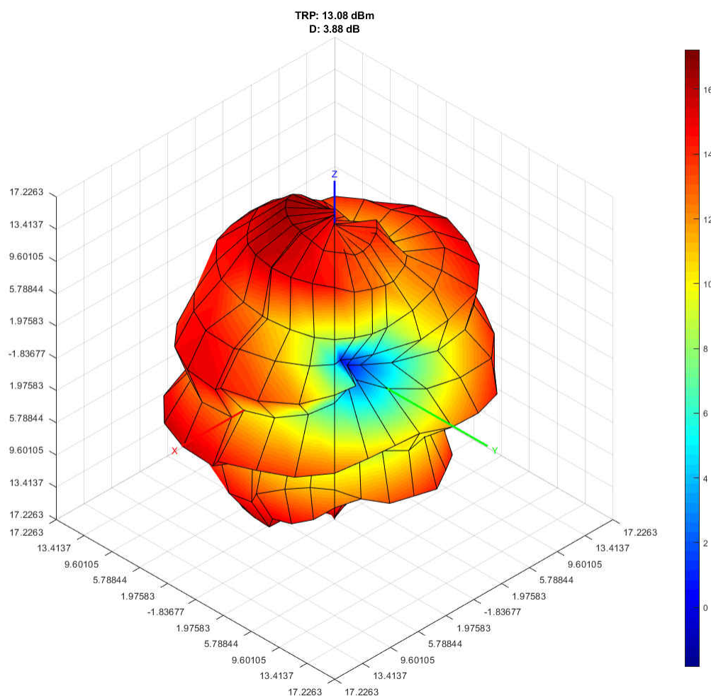
Figure 5-30. Radiation Pattern of the Antenna Matched for Dual-Band 868/915 and 2440-MHz Radiating with 13-dBm 915-MHz Setting
