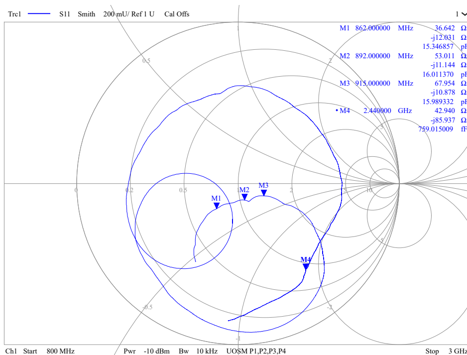
Figure 3-11. Smith Chart After placing a 2-pF Capacitor on Z64.
