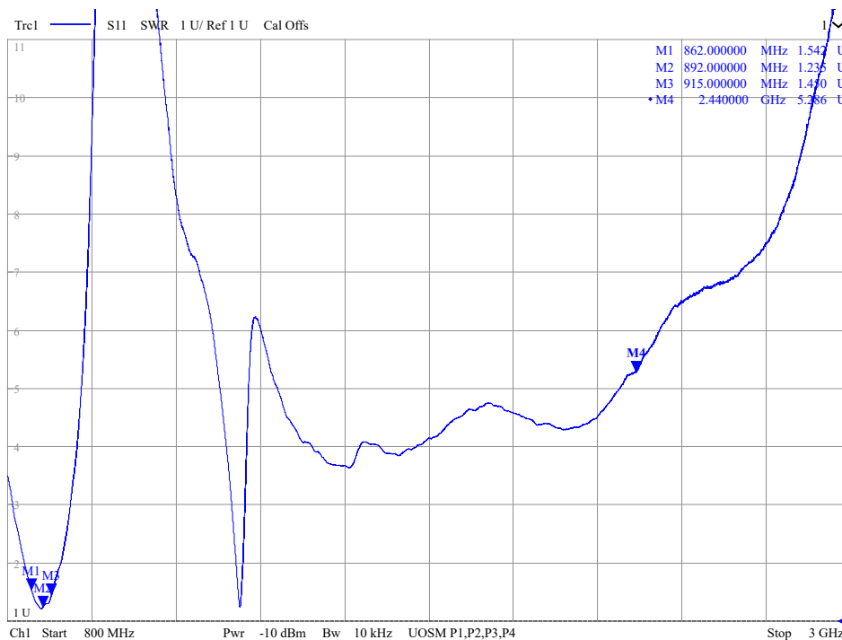
Figure 3-12. SWR After Placing a 2-pF Capacitor on Z64.
