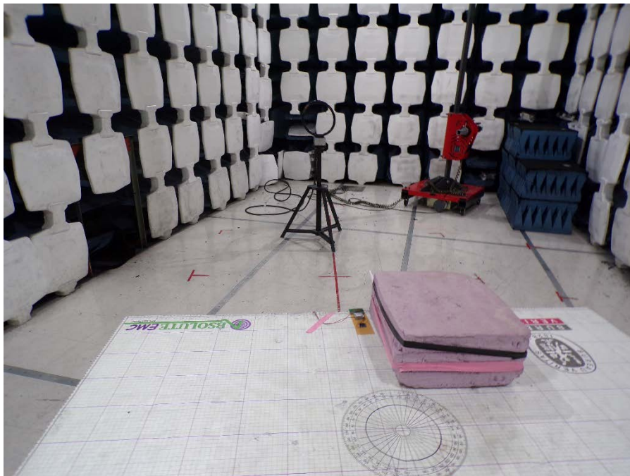
1-30MHz Radiated Spurious Back
