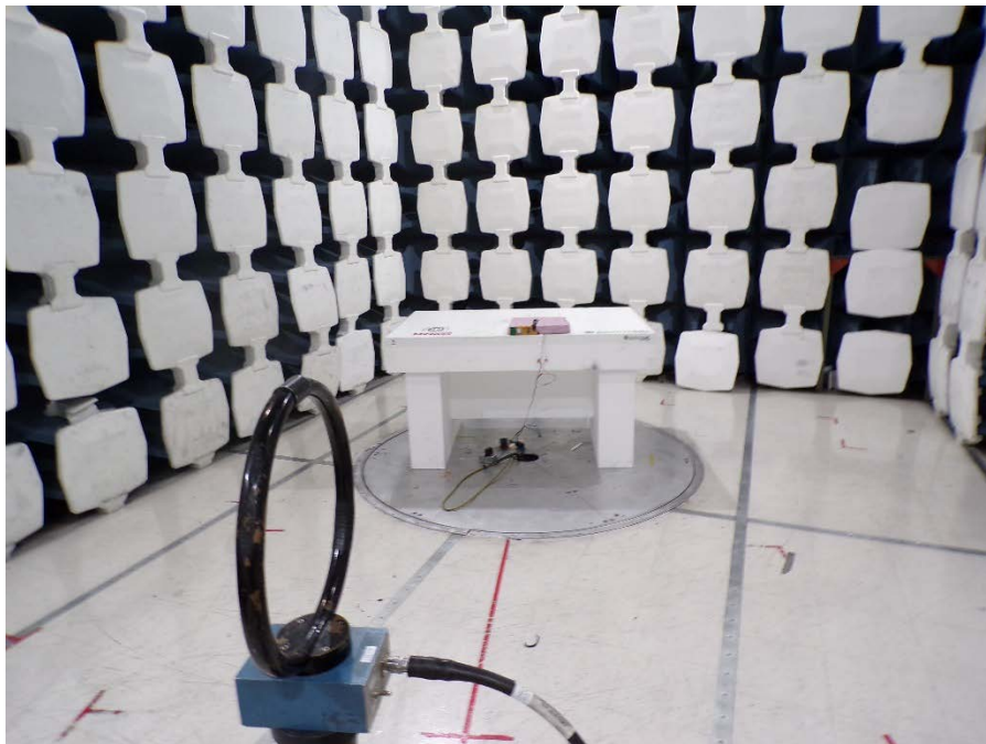
1-30MHz Radiated Spurious Front
