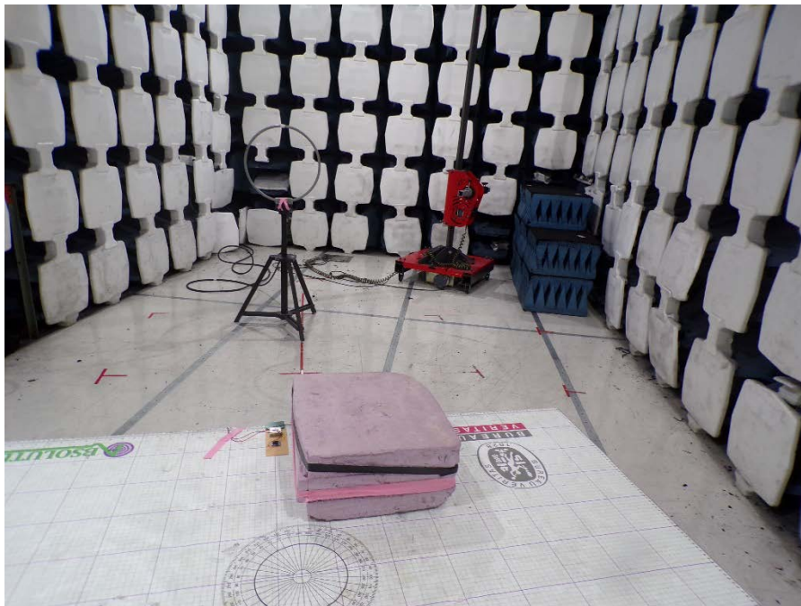
0.009-1MHz Radiated Spurious Back
