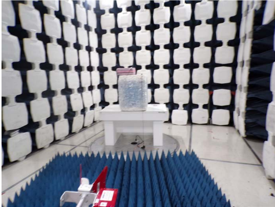
1-10GHz Radiated Spurious Front
