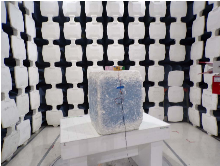
18-25GHz Radiated Spurious
