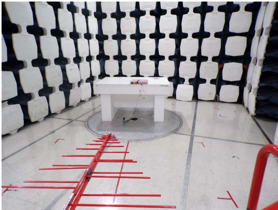
30-1000MHz Radiated Spurious Front
