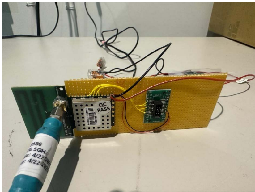
Internal Antenna Closeup
