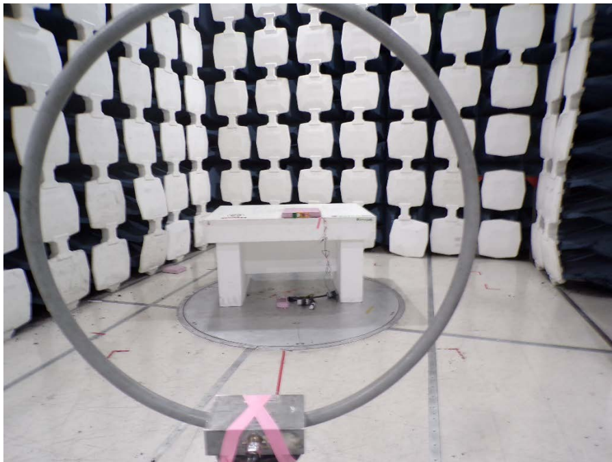
0.009-1MHz Radiated Spurious Front
