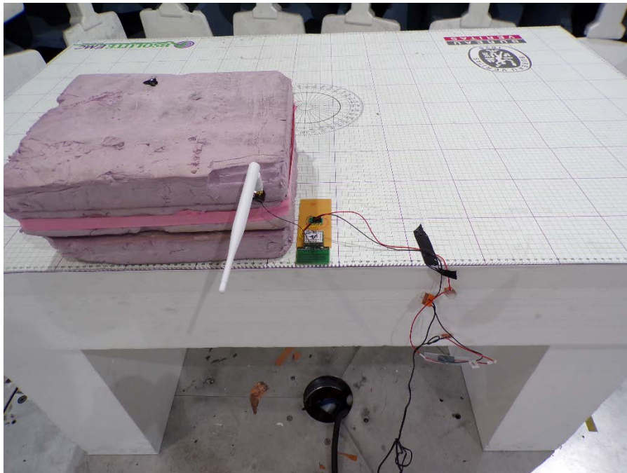
Module: Z-Axis External Antenna: Horizontal (Worst Case Orientation)
