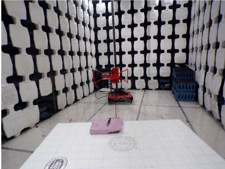
30-1000MHz Radiated Spurious Back
