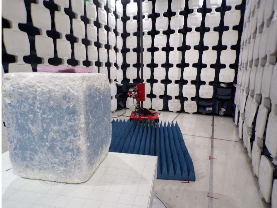
1-18GHz Radiated Spurious Back
