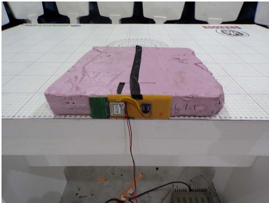
Module: Y-Axis (Worst Case Orientation)
